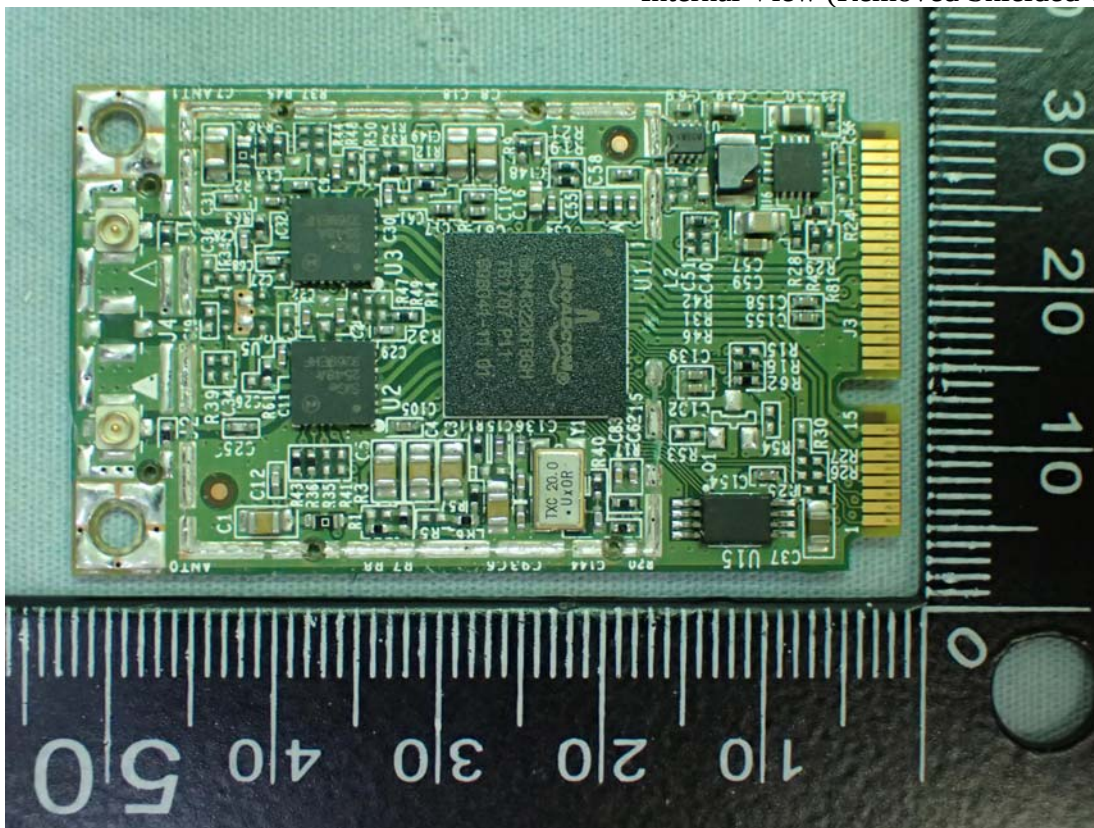
Figure 9 Internal View (Removed Shielded Cover)
