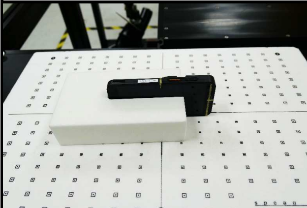
Left Side of EUT Tested at 0 mm
