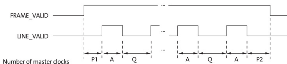
Figure 15. Row Timing and FRAME_VALID/LINE_VALID Signals
