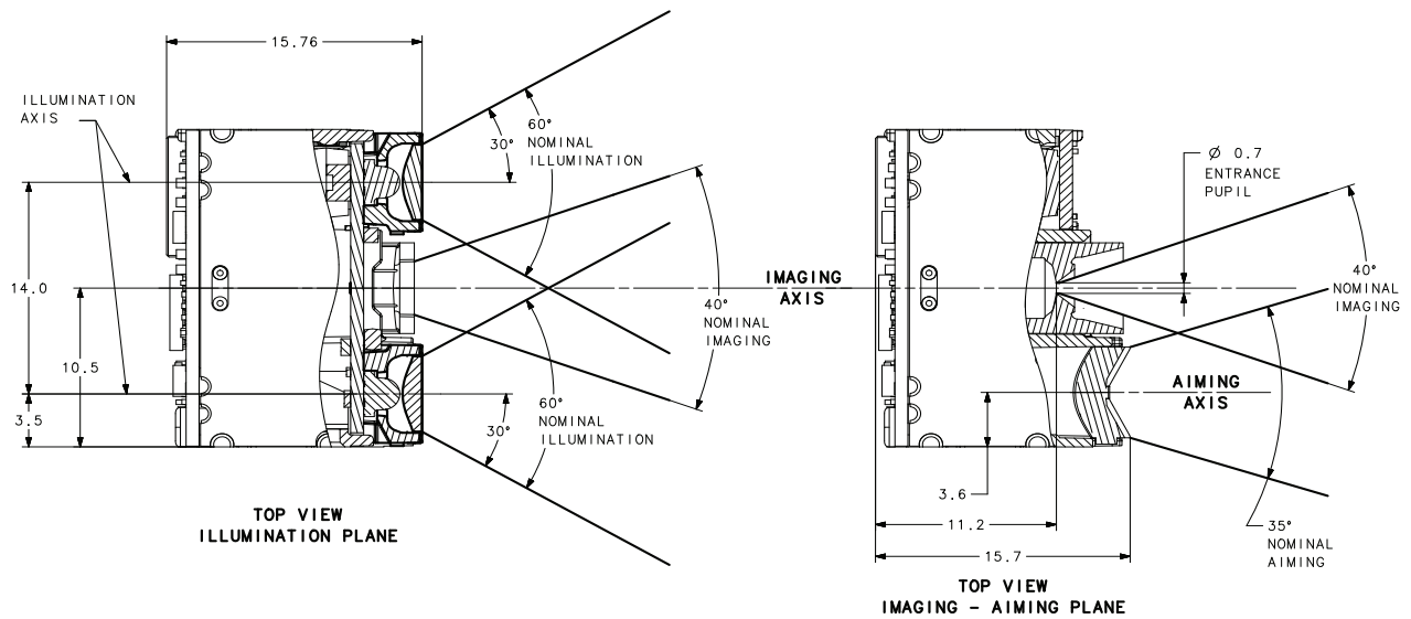
Figure 8. Top view - Aiming, imaging and illumination optical paths
