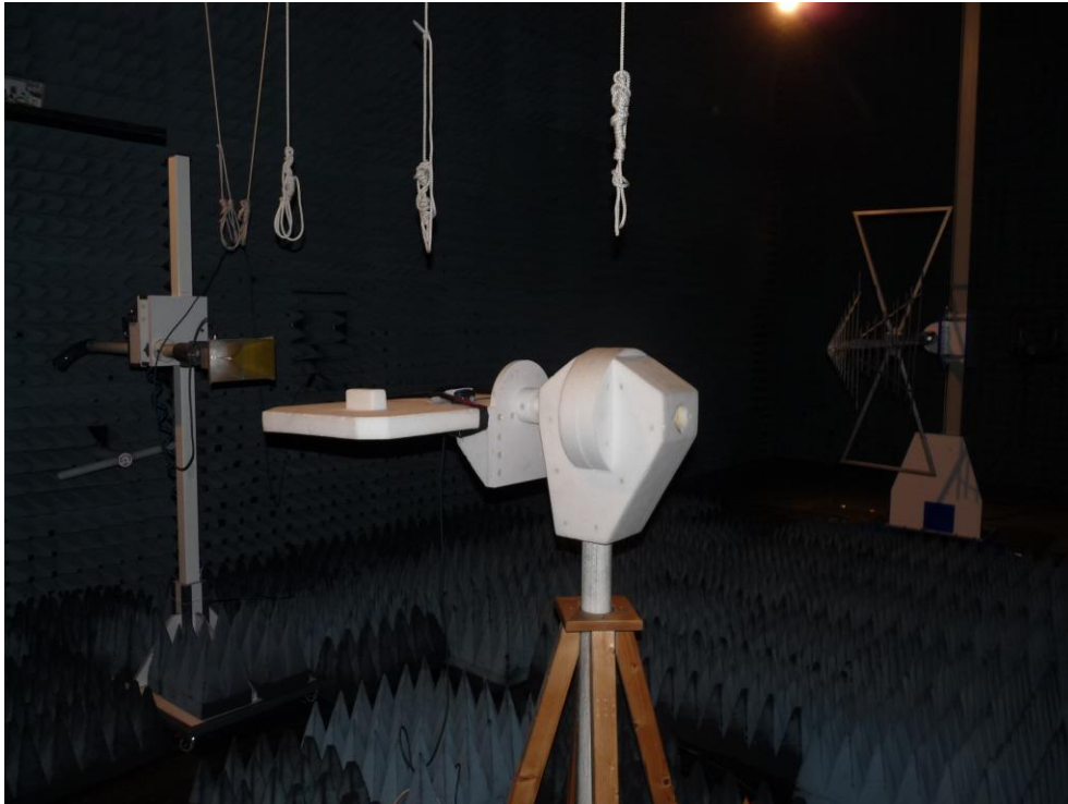
Photo 1: Test setup for radiated measurements (1 GHz to 18 GHz)
