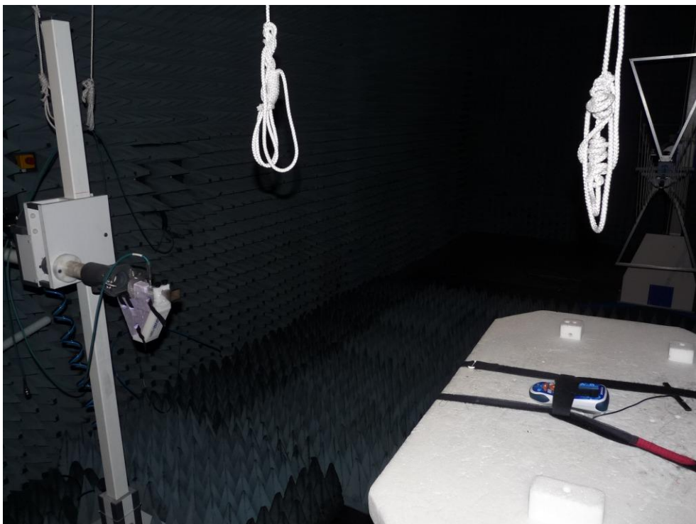
Photo 2: Test setup for radiated measurements (18 GHz to 25 GHz)
