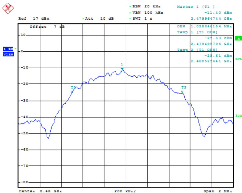
Fig.26 99% Bandwidth: Ch19
