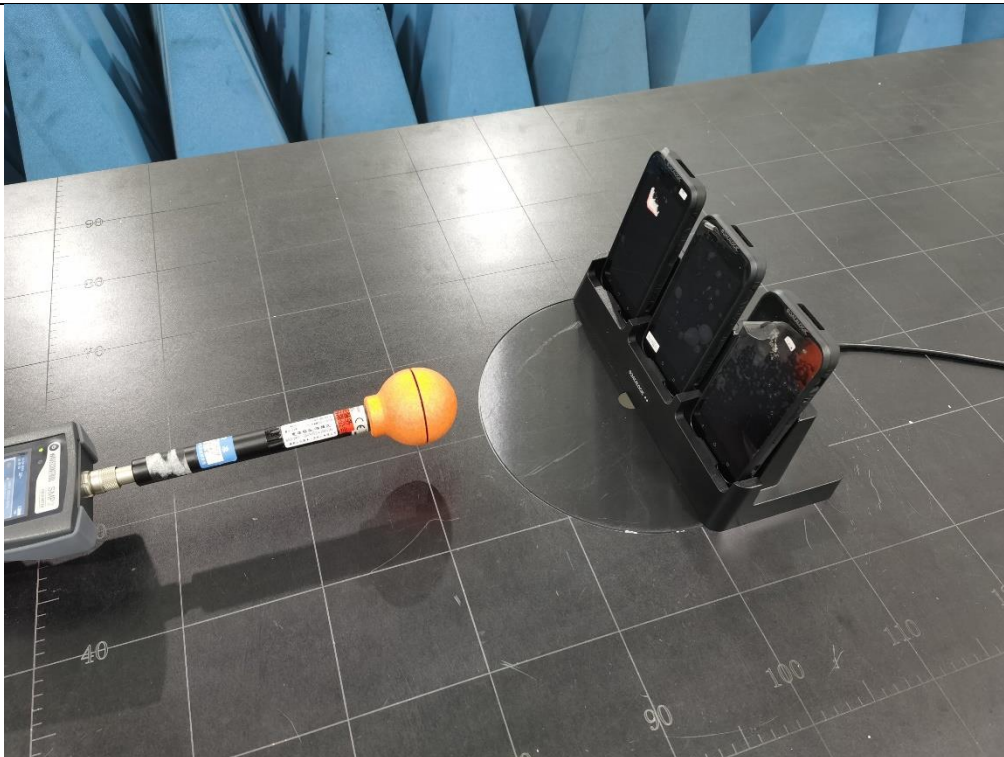
Description: RF Exposure Setup –Above 100kHz
