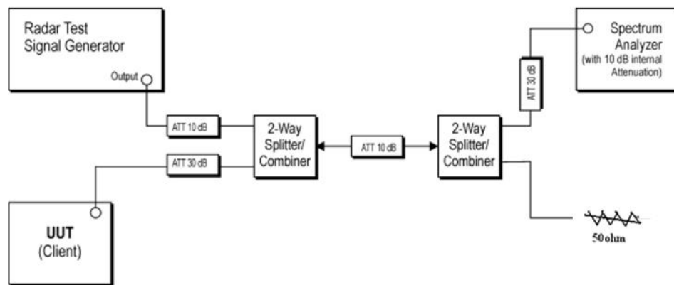
Figure 3-2: Conducted Test Setup
