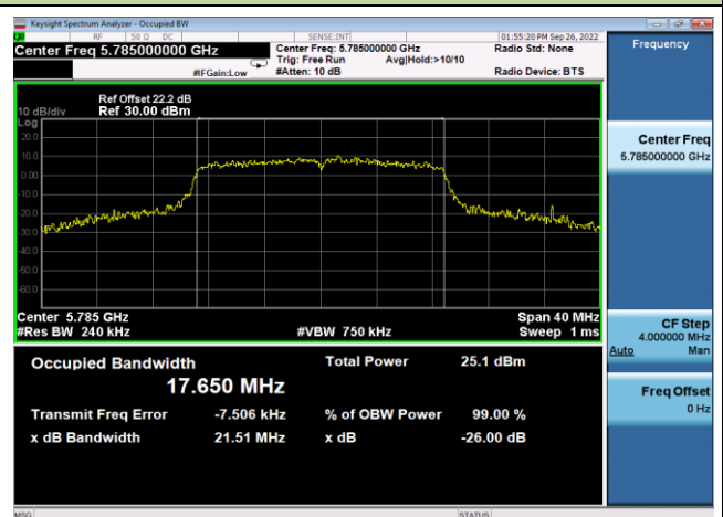
Channel 157 (5785MHz)
