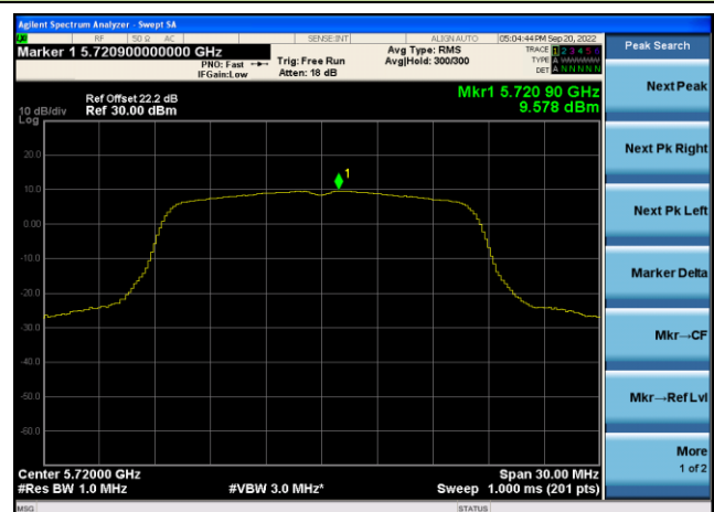
Channel 144 (5720MHz)
