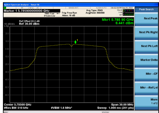
Channel 157 (5785MHz)
