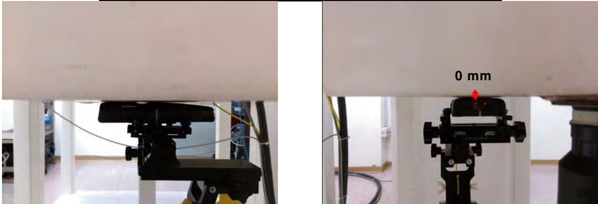
Fig.9 EUT Back side to flat phantom
