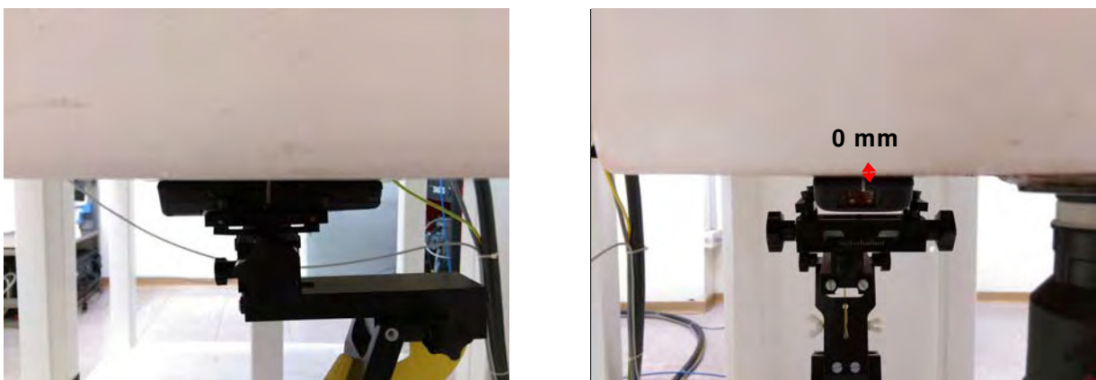
Fig.11 EUT Front side to flat phantom
