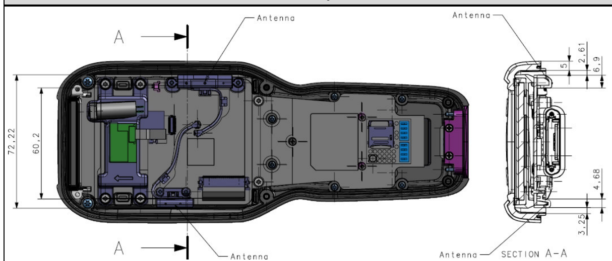
EUT Antenna position
