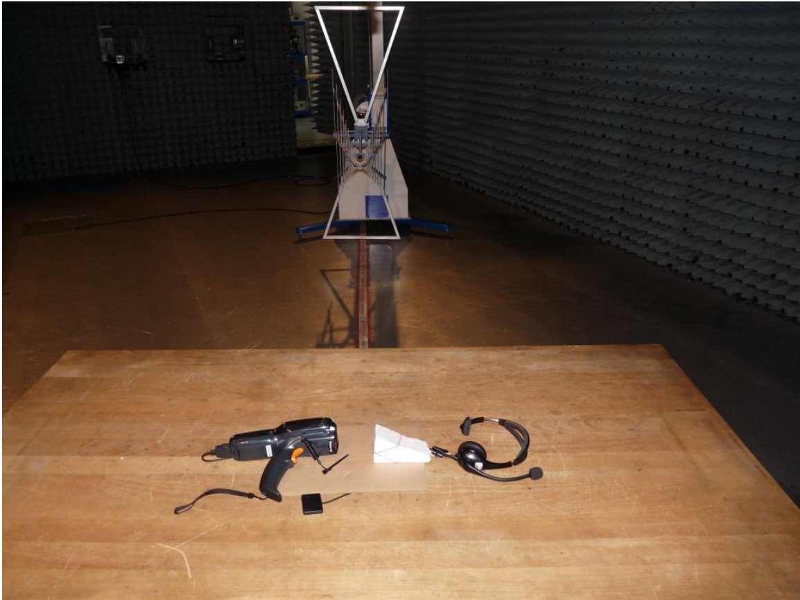
Photo 6: Test setup for radiated measurements (unintentional radiator §15), rear view, Setup AB01
