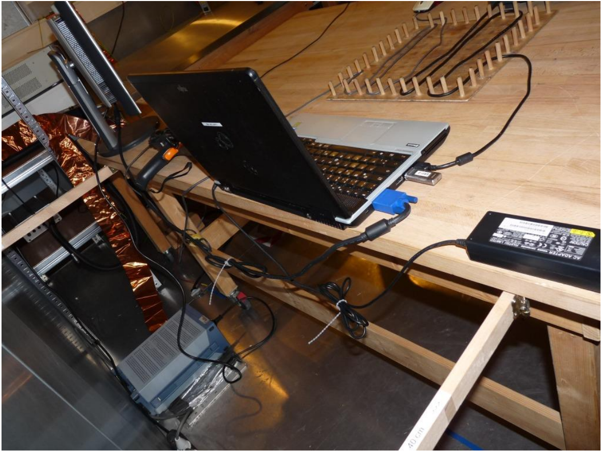
Photo 2: Test setup for conducted measurements (AC Port (power line), unintentional radiator §15) , Setup AA01
