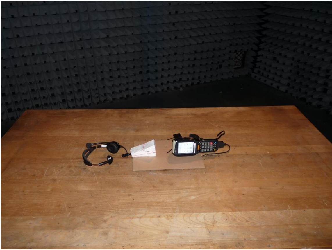
Photo 5: Test setup for radiated measurements (unintentional radiator §15), front view, Setup AB01
