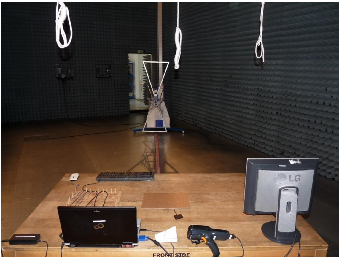
Photo 4: Test setup for radiated measurements (unintentional radiator §15), rear view, Setup AA01
