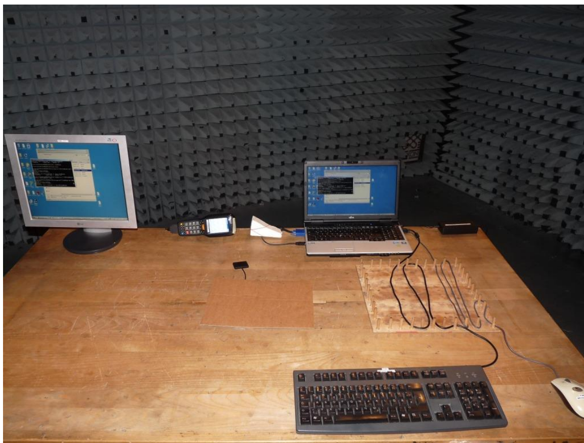
Photo 3: Test setup for radiated measurements (unintentional radiator §15), front view, Setup AA01
