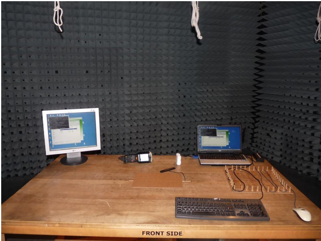
Photo 1: Test setup for radiated measurements (unintentional radiator §15)
