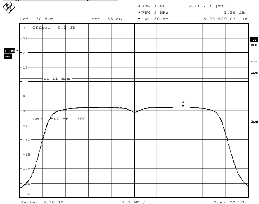
Diagram a-Mode 24Mbps Ch56:
