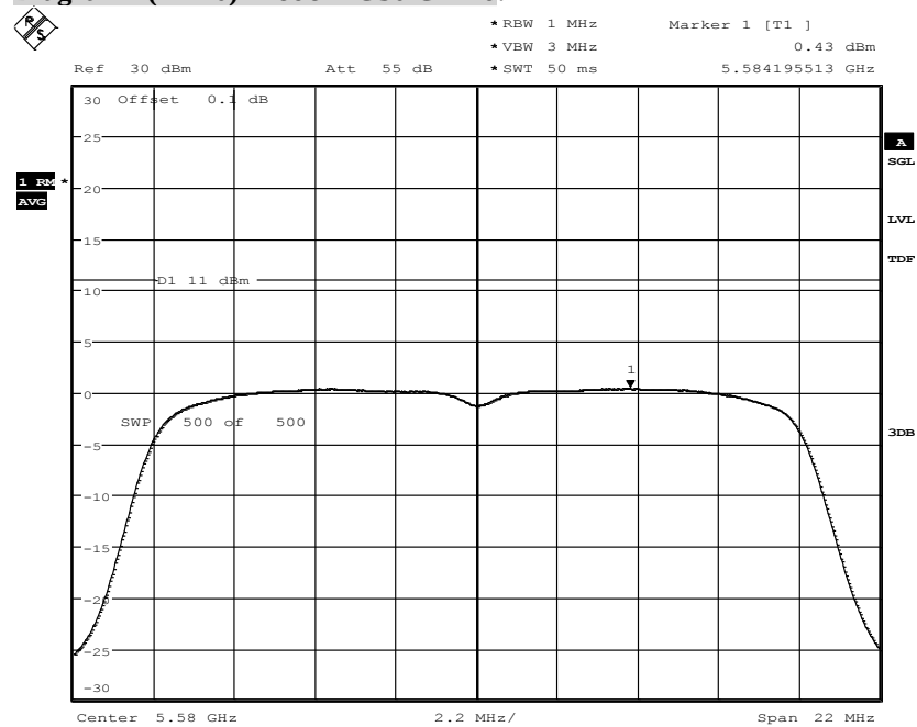
Diagram n(HT20)-Mode MCS0 Ch116:
