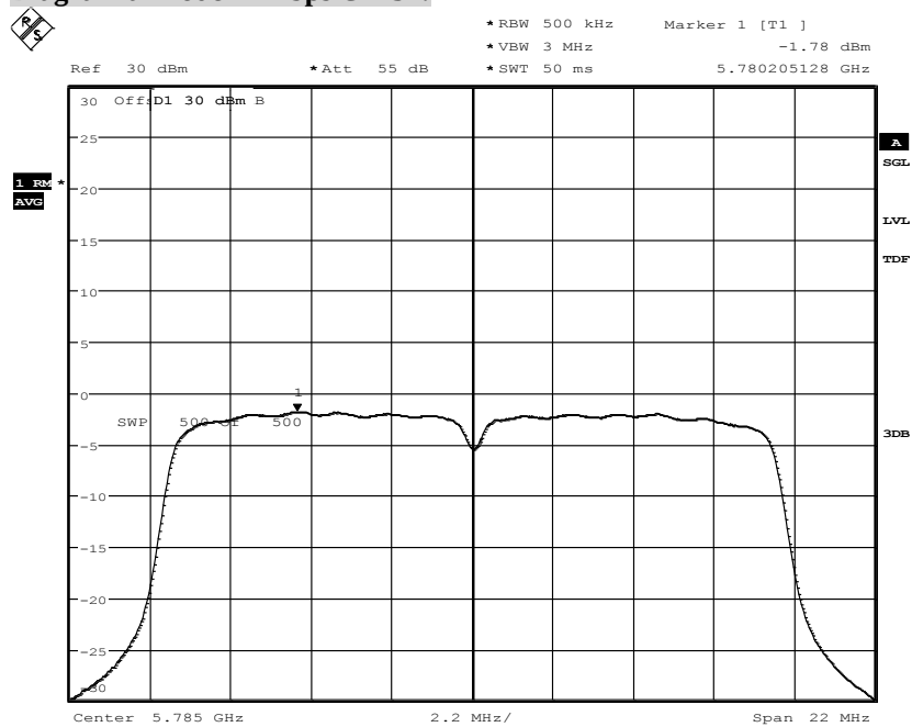
Diagram a-Mode 24Mbps Ch157:
