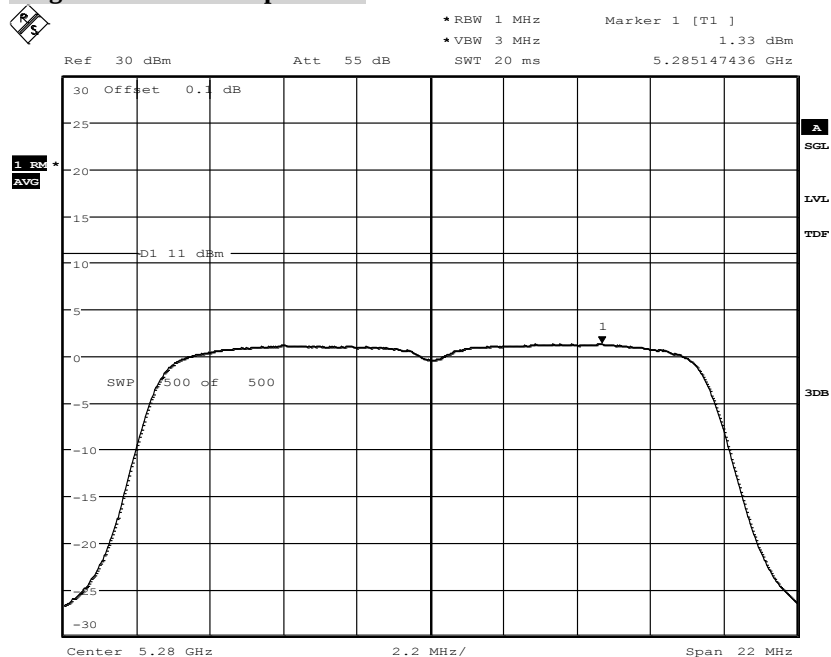
Diagram a-Mode 6Mbps Ch56:
