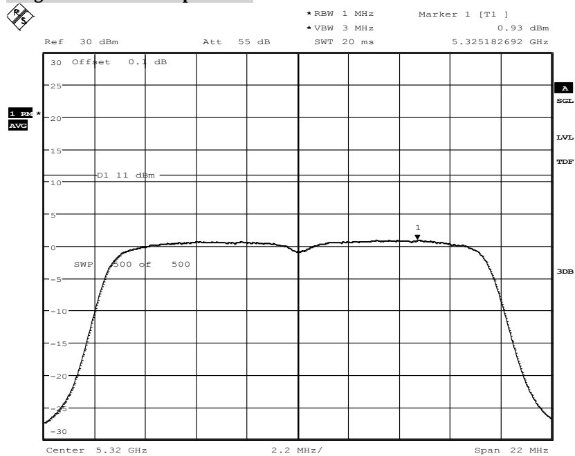
Diagram a-Mode 6Mbps Ch64:
