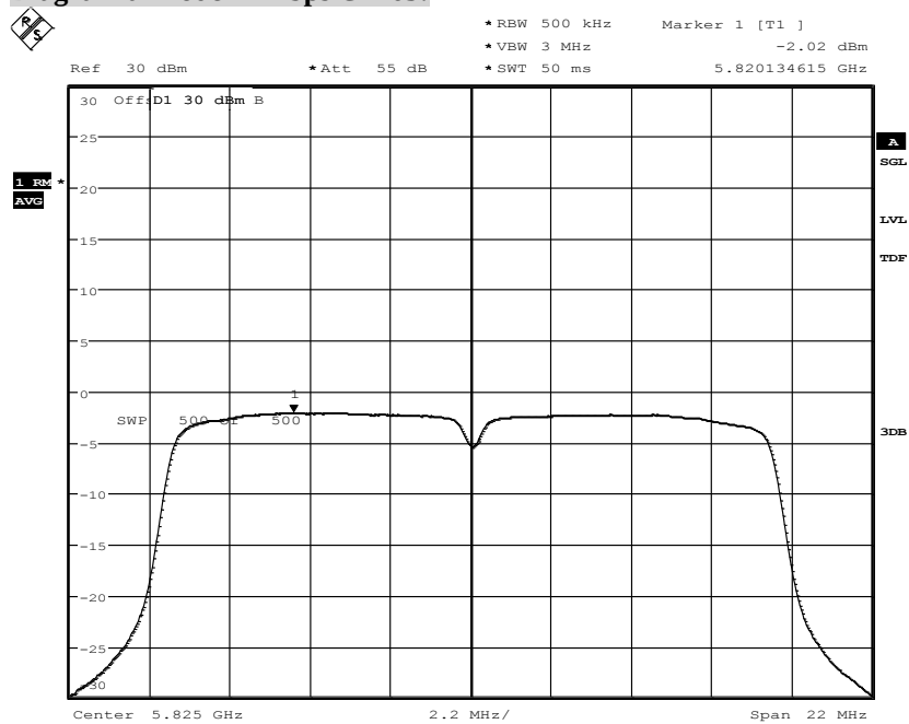
Diagram a-Mode 12Mbps Ch165:
