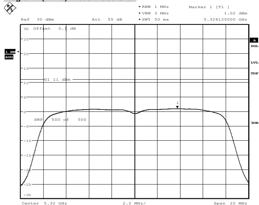
Diagram n(HT20)-Mode MCS0 Ch64:
