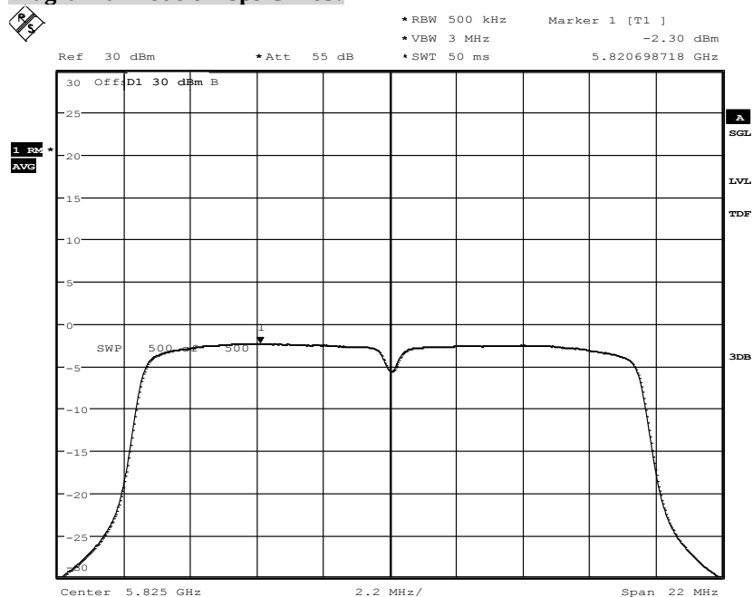
Diagram a-Mode 6Mbps Ch165:
