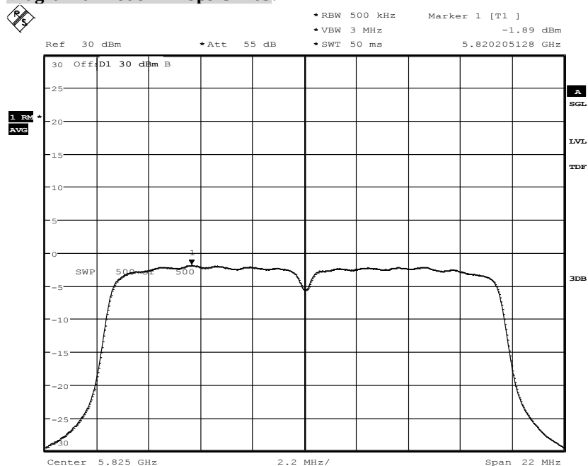
Diagram a-Mode 24Mbps Ch165:
