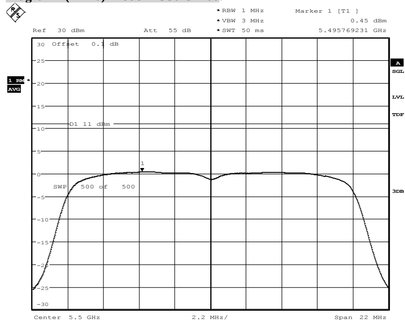
Diagram n(HT20)-Mode MCS0 Ch100:
