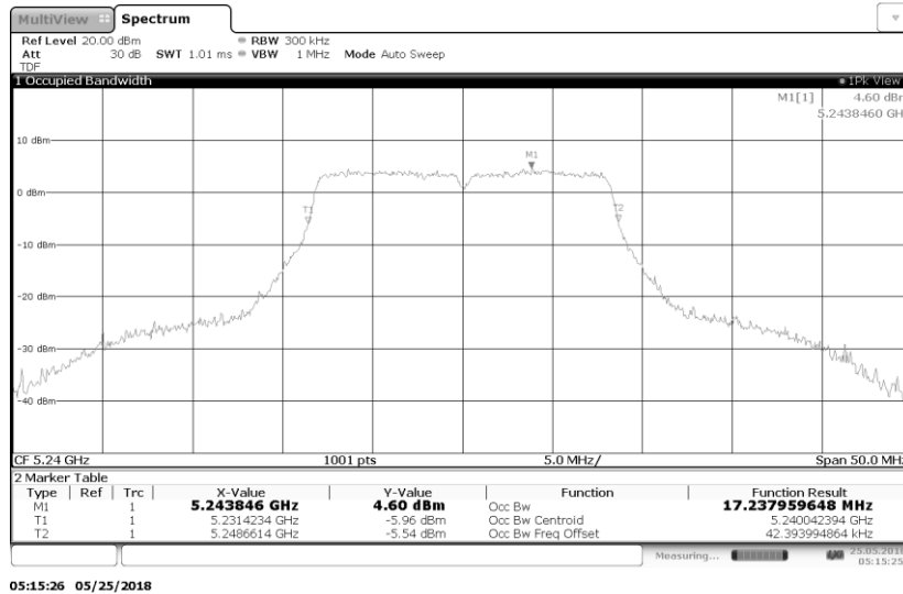
Diagram 5: 35.01_OBW_Ch48_A_Mode_18MBit
