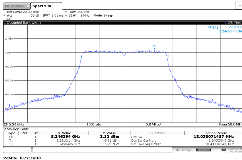
Diagram 6: 35.02_OBW_CH48_N_Mode_MCS4
