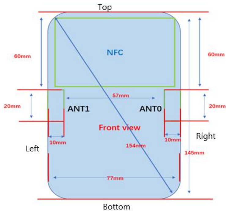
Photo 5: Antenna position
