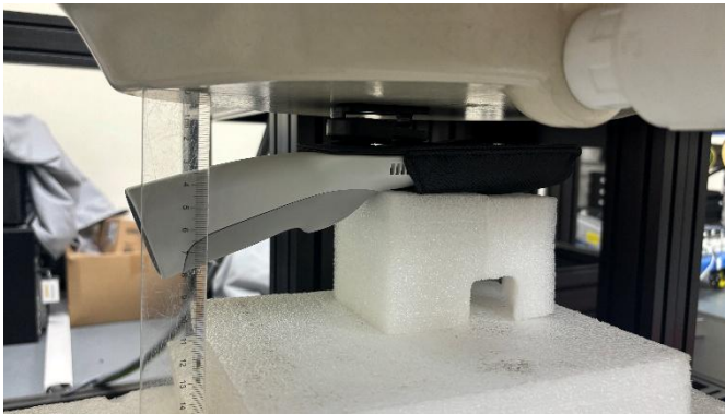
Front Surface-Parallel back clip(0mm)
