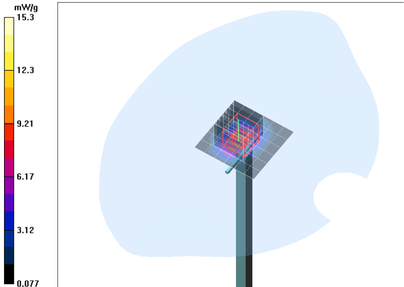
Fig. 4: Validation measurement 2450 MHz Body (July 11, 2014), coarse grid.
