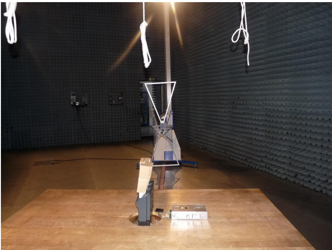
Photo 4: Test setup for radiated measurements, (unintentional radiator §15) 3-slot-cradle setup
