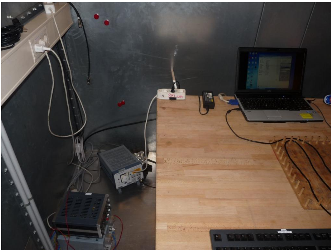
Photo 2: Test setup for conducted measurements, unintentional radiator (§15) single device setup, computer peripheral setup.
