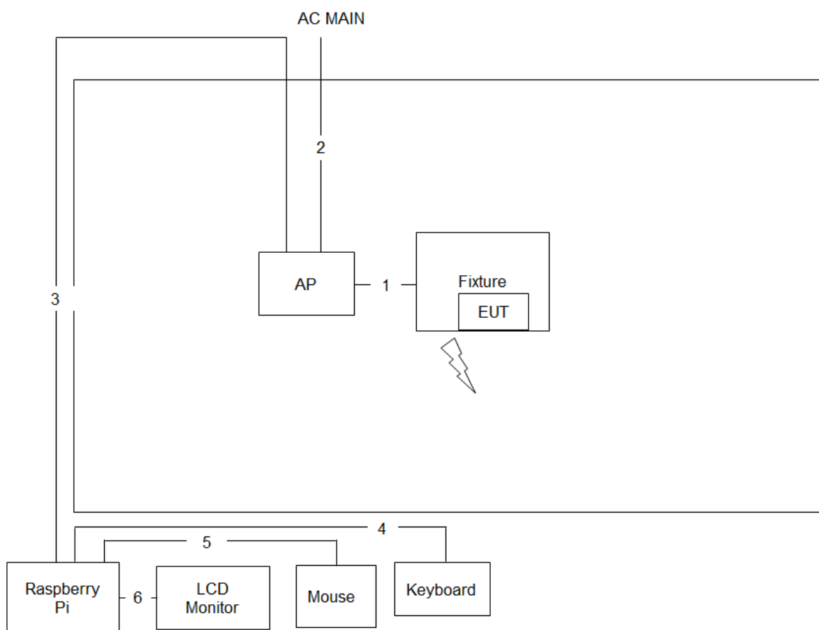
Test Setup Diagram - Radiated Test
