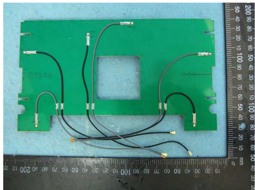
Antenna backside view
