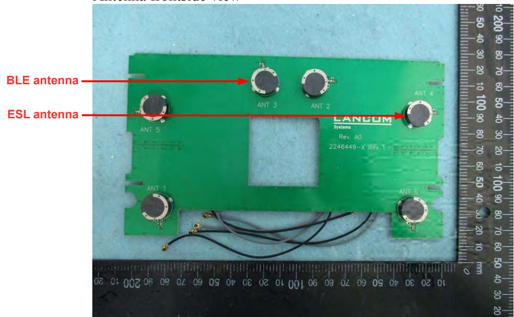
Antenna frontside view
