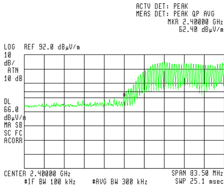
Figure 11 — 2400.0 MHz
