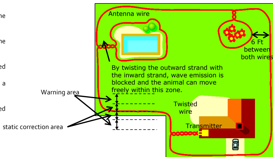
Diagram 4 – Sample installation
