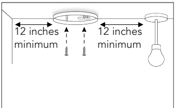
Figure 3 Position CO Alarm
