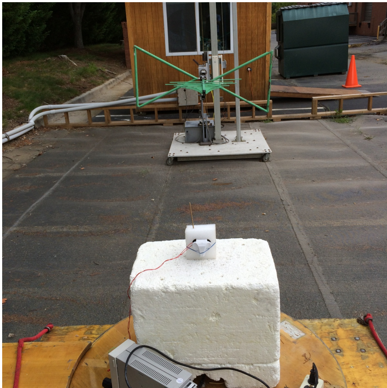
Radiated Emissions
