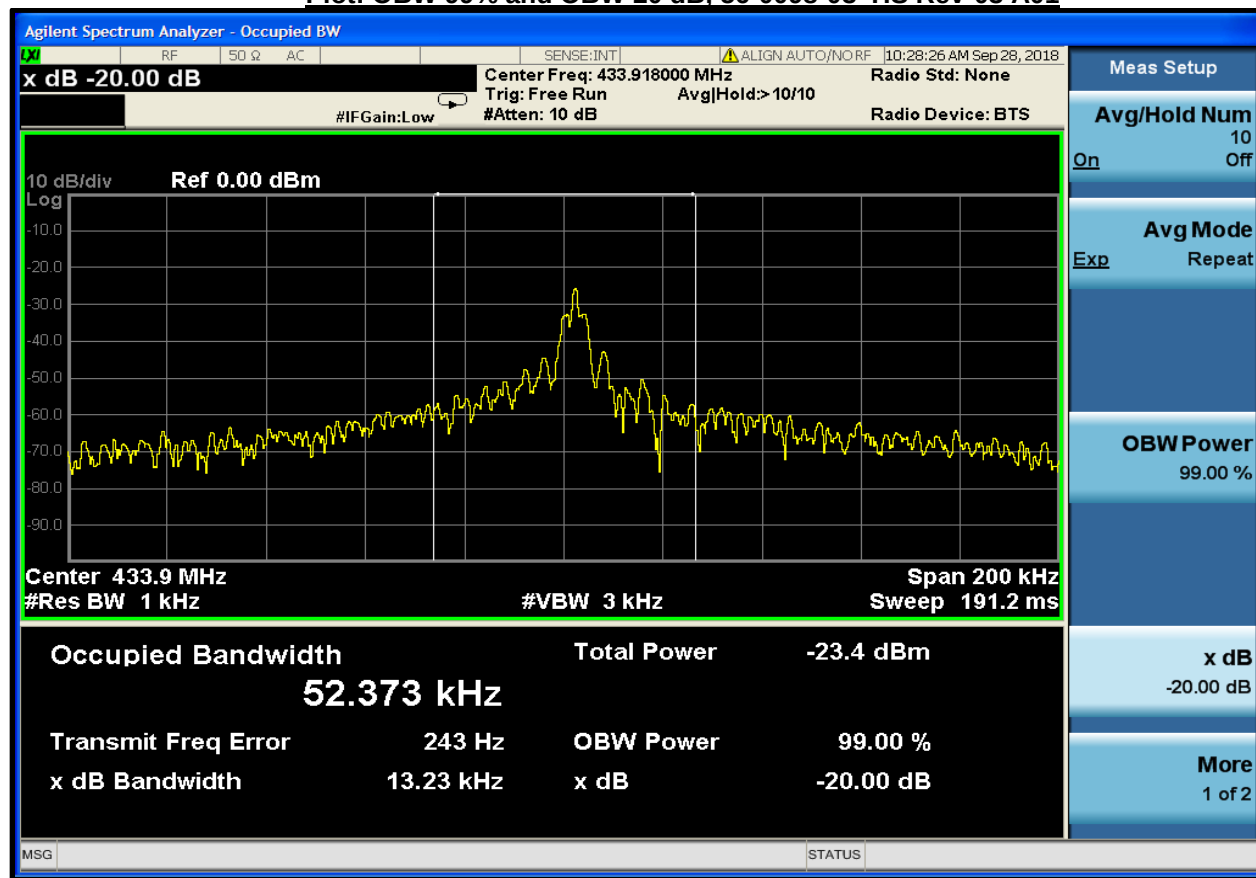
Plot: OBW 99% and OBW 20 dB, 56-0098-03_HS Rev-03 A01
