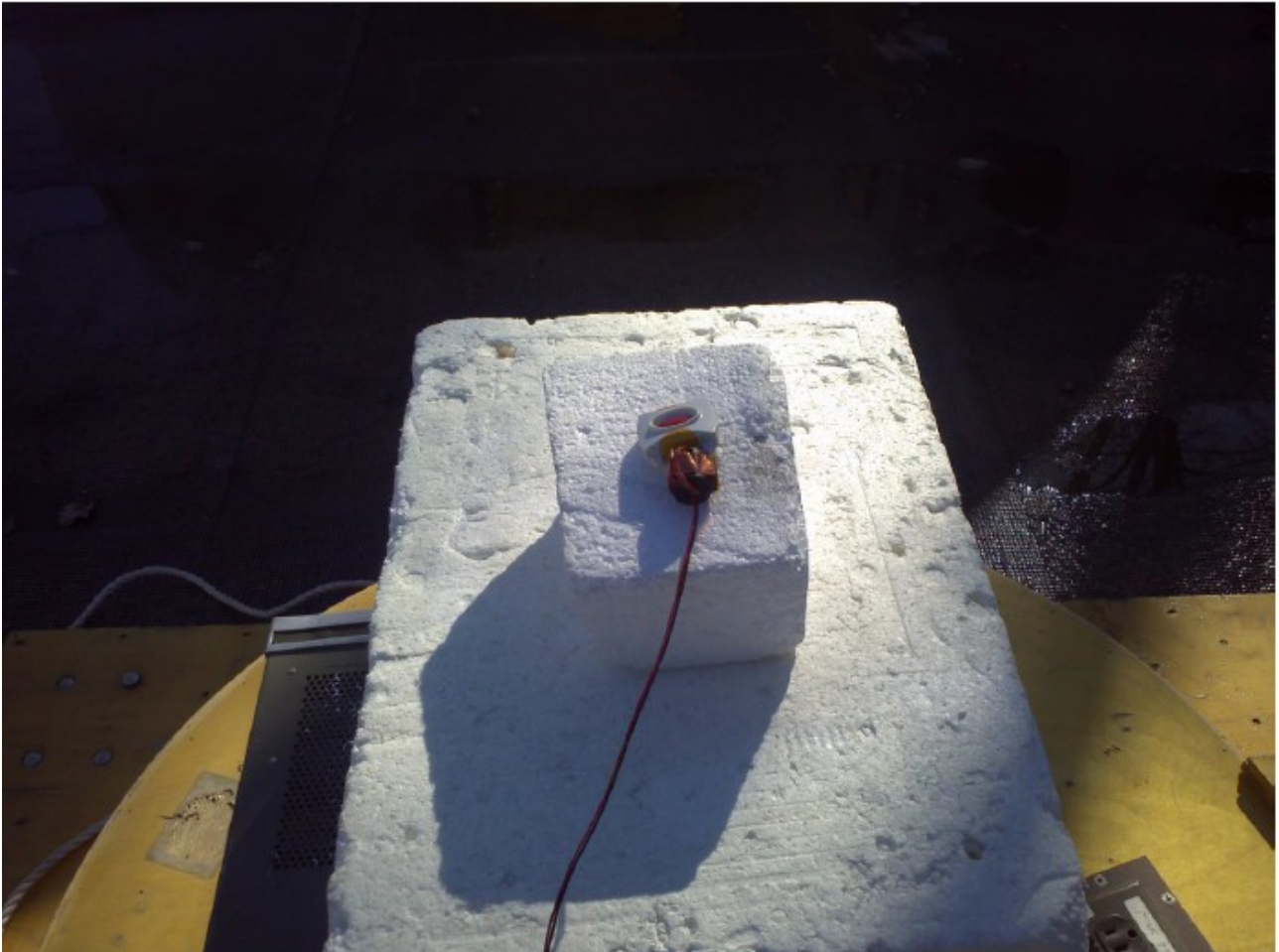
Radiated Emissions
