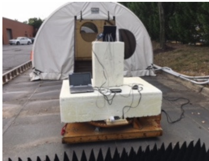
Radiated Emissions (Front View) > 1 GHz
