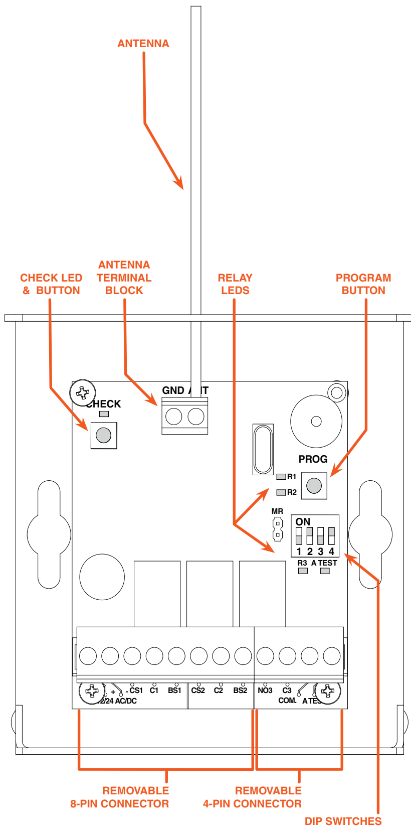
IMAGE 2. RBAND GATE EDGE RECEIVER PCB & CONNECTIONS
