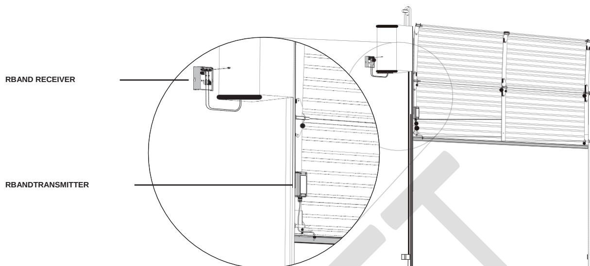
RBAND-PROX COMMERCIAL DOOR INSTALLATION
