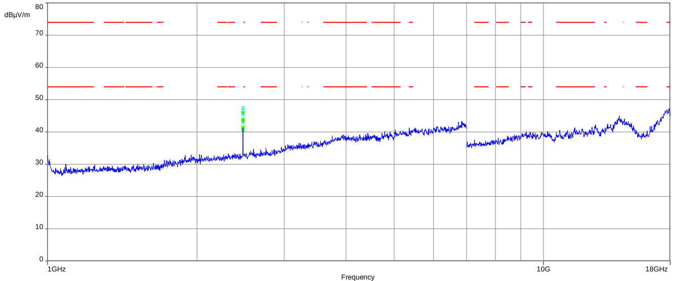
Plot 3: 1 GHz to 18 GHz, RX / idle – mode, highest channel, vertical & horizontal polarization
