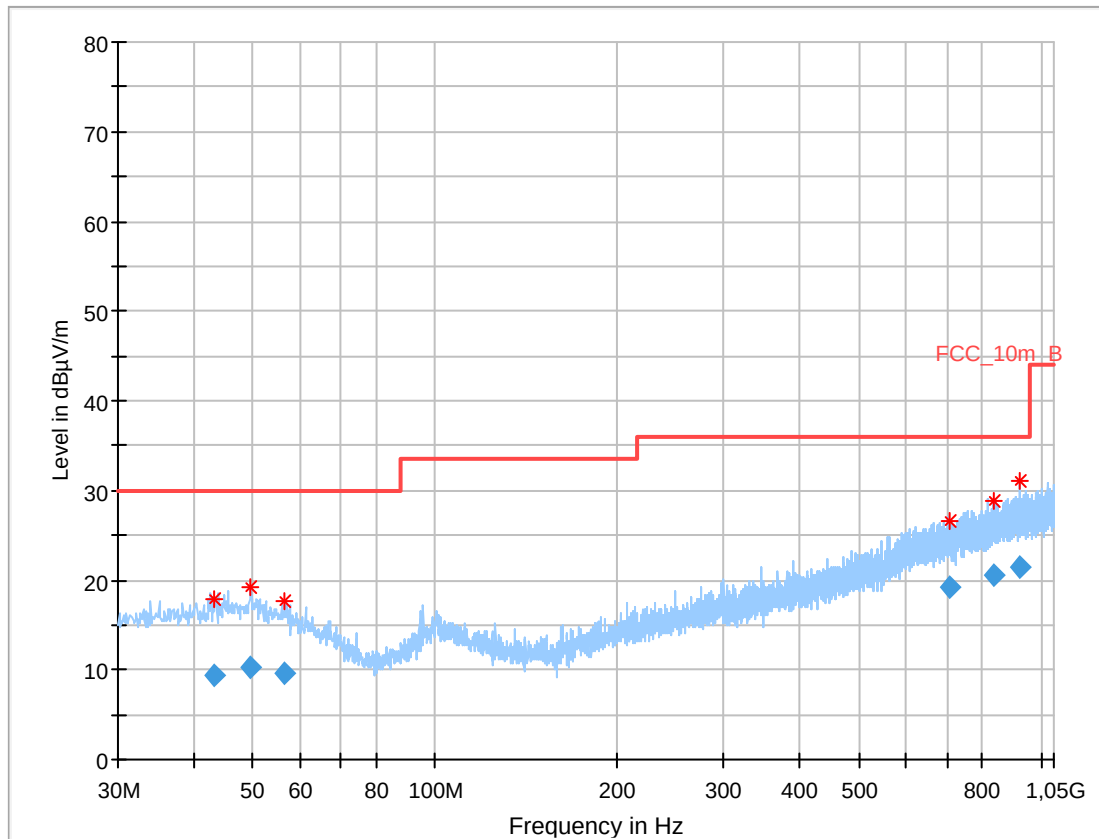
Plot 2: 30 MHz to 1 GHz, RX mode, highest channel, vertical & horizontal polarization
