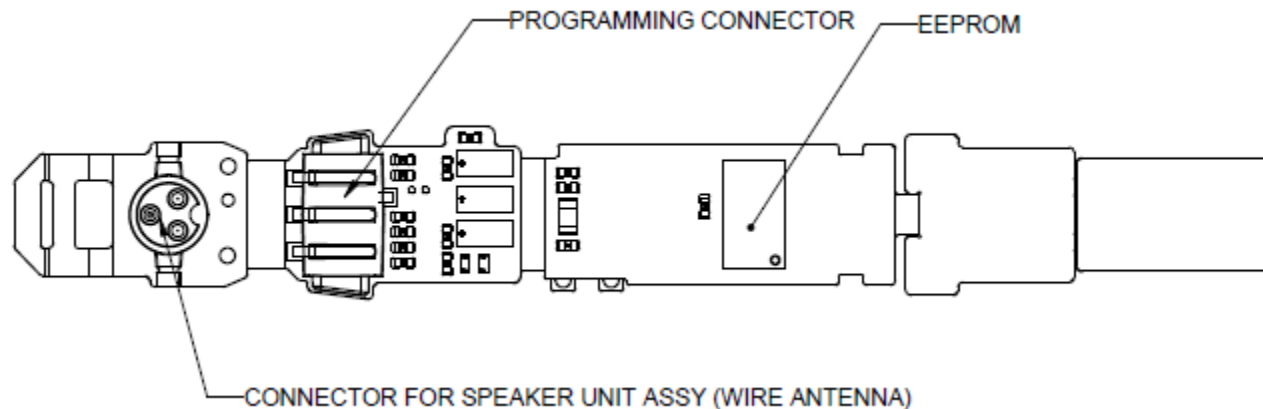
Aurora miniRITE 312 T Rc Radio Model – Main PCB – Bottom side
