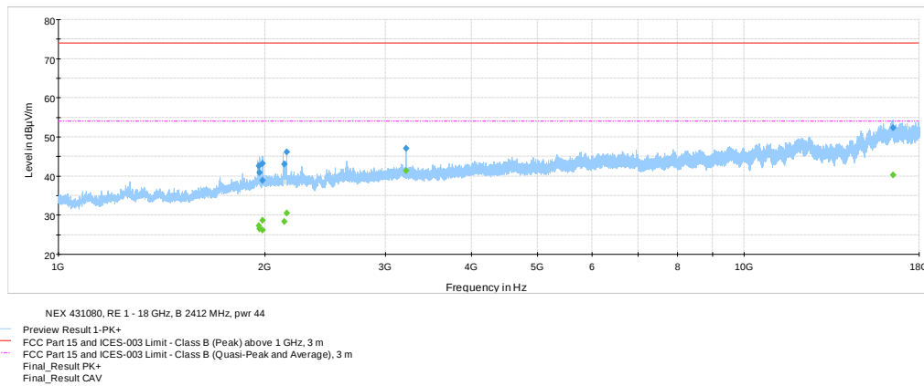
Figure 8.7-12: Radiated spurious emissions 1 – 18 GHz on 802.11b @ 2412 MHz
