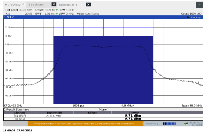
Figure 8.6-2: Conducted output power on 802.11g, sample plot
