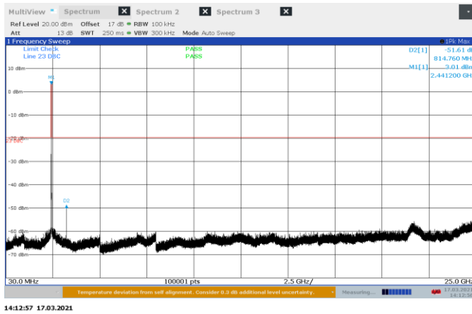
Figure 8.7-28: Conducted spurious emissions on 802.11b, Port A 2442 MHz
