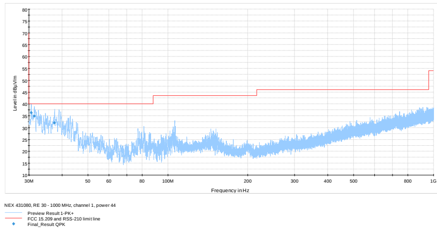
Figure 8.7-9: Radiated spurious emissions 30 – 1000 MHz on 802.11b @ 2412 MHz
