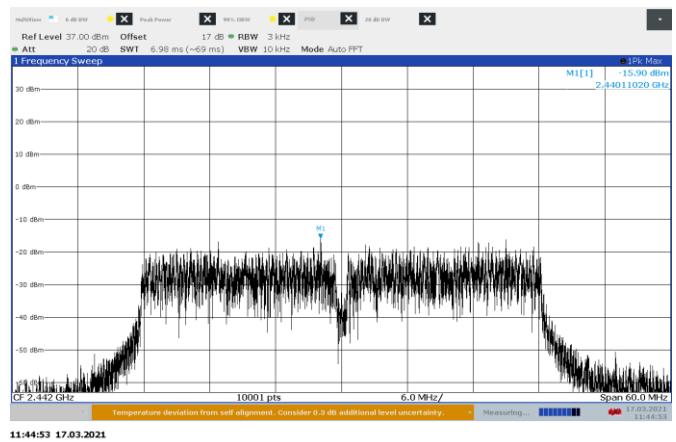
Figure 8.8-4: Conducted PSD on 802.11n HT40, sample plot
