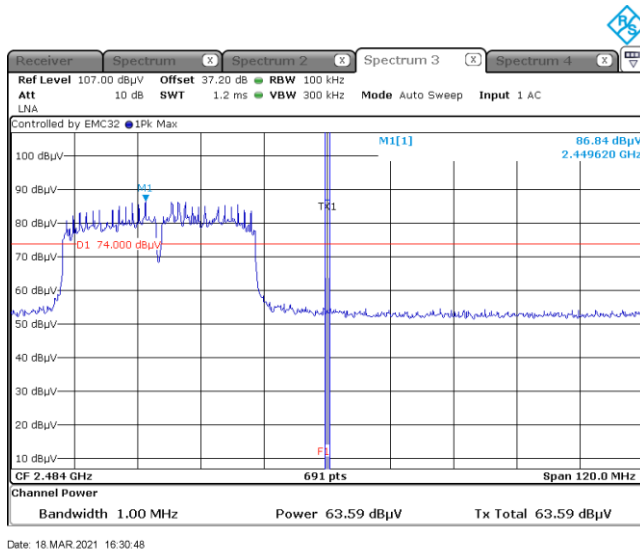
Figure 8.7-3: Radiated restricted-band band edge at 2483.5 MHz, 802.11n HT40 Peak
