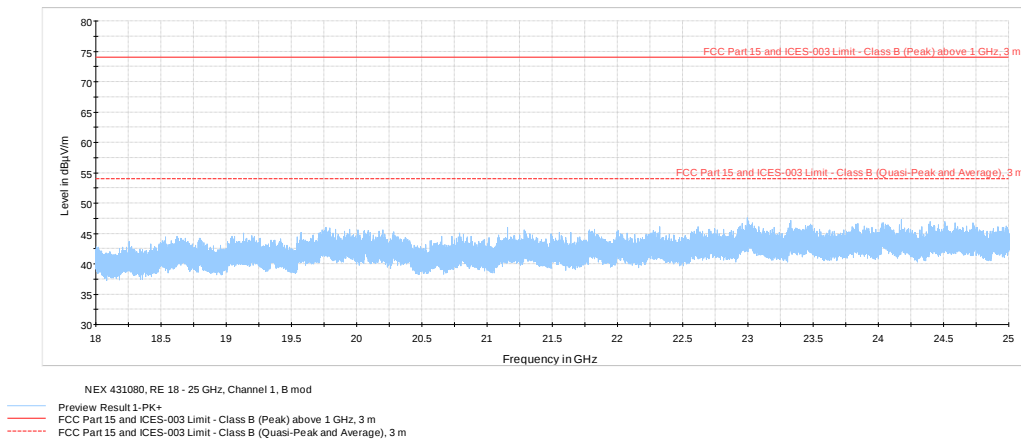
Figure 8.7-15: Radiated spurious emissions 18 – 25 GHz on 802.11b @ 2412 MHz
