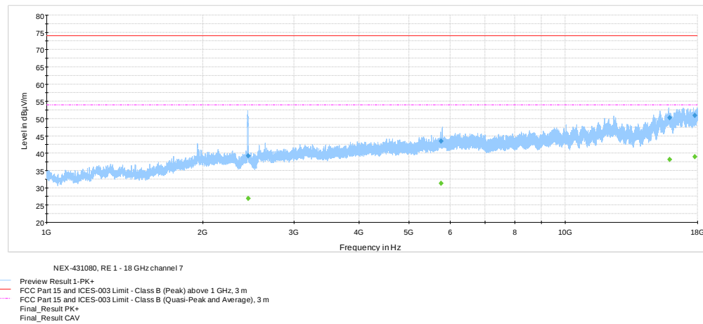
Figure 8.7-13: Radiated spurious emissions 1 – 18 GHz on 802.11b @ 2442 MHz
