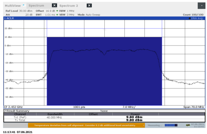
Figure 8.6-4: Conducted output power on 802.11n HT40, sample plot
