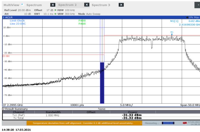
Figure 8.7-24: Conducted Band edge spurious emissions at 2400 MHz, 802.11g Port B
