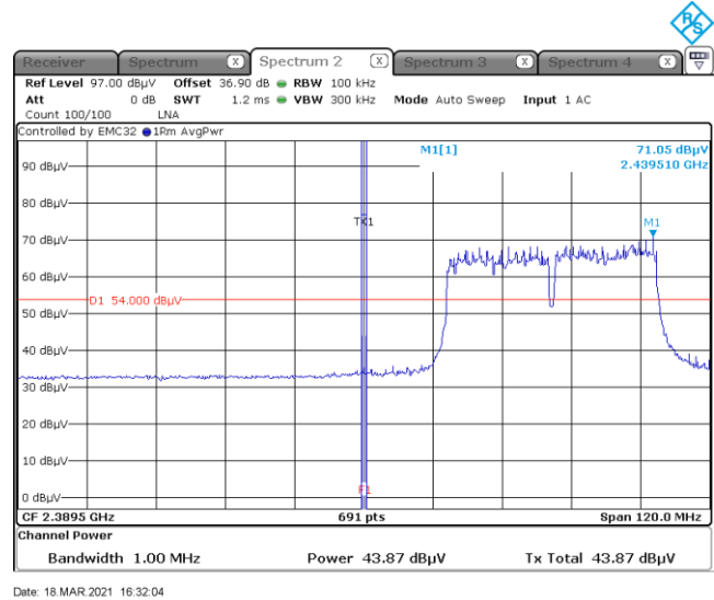
Figure 8.7-2: Radiated restricted-band band edge at 2390 MHz, 802.11n HT40 Average
