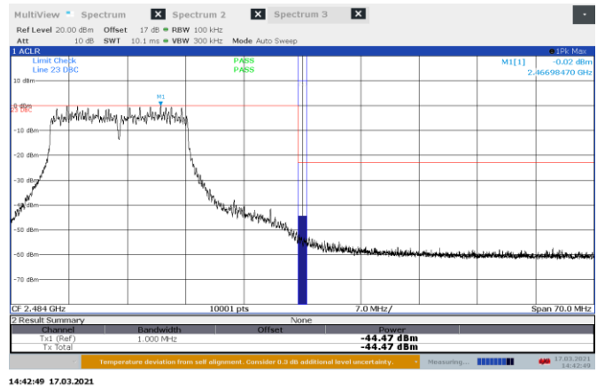
Figure 8.7-23: Conducted Band edge spurious emissions at 2483.5 MHz, 802.11g Port A
