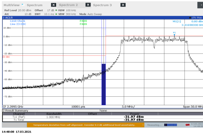
Figure 8.7-22: Conducted Band edge spurious emissions at 2400 MHz, 802.11g Port A
