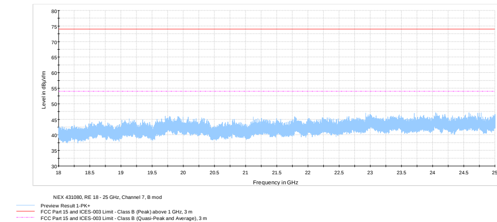
Figure 8.7-16: Radiated spurious emissions 18 – 25 GHz on 802.11b @ 2442 MHz
