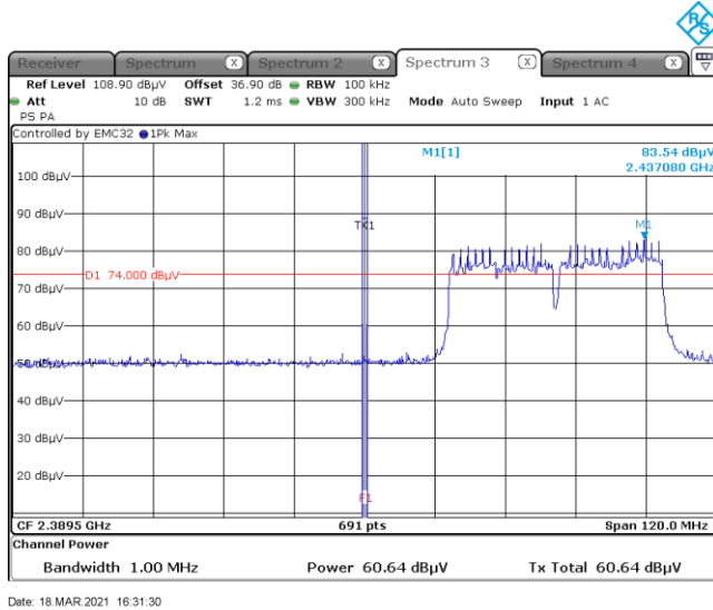
Figure 8.7-1: Radiated restricted-band band edge at 2390 MHz, 802.11n HT40 Peak
