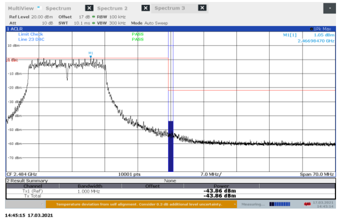
Figure 8.7-25: Conducted Band edge spurious emissions at 2483.5 MHz, 802.11g Port B
