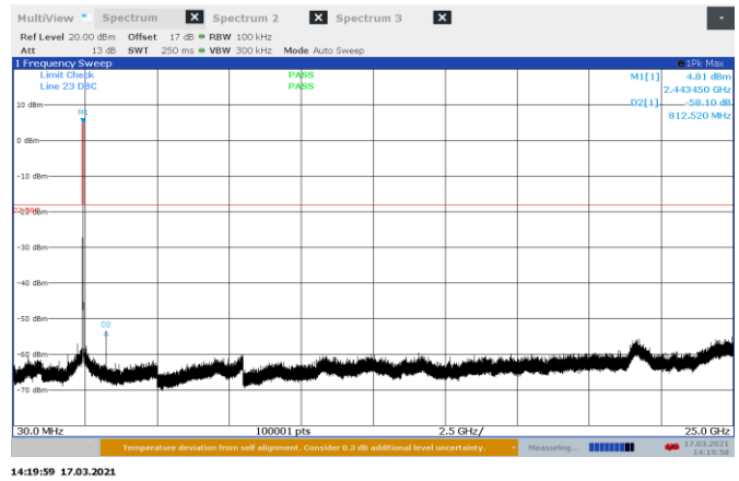
Figure 8.7-29: Conducted spurious emissions on 802.11b, Port B 2442 MHz
