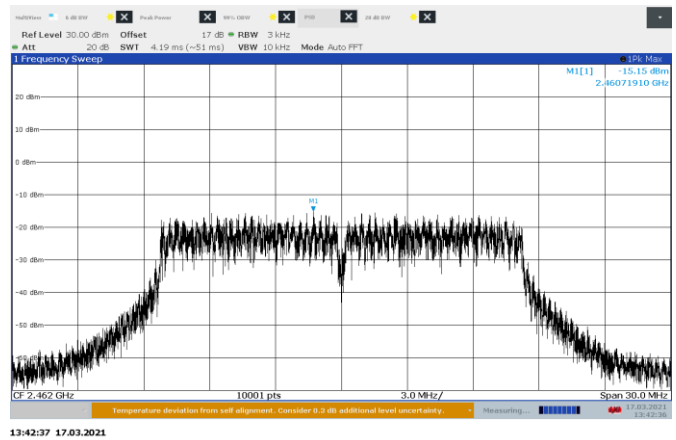
Figure 8.8-2: Conducted PSD on 802.11g, sample plot
