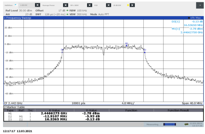
Figure 8.5-2: 6 dB bandwidth on 802.11g, sample plot
