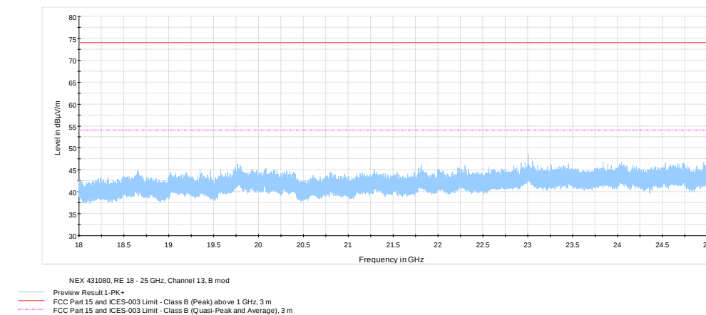
Figure 8.7-17: Radiated spurious emissions 18 – 25 GHz on 802.11b @ 2472 MHz
