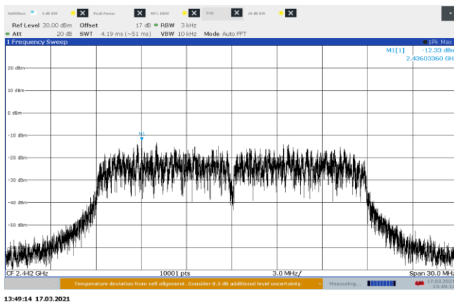
Figure 8.8-3: Conducted PSD on 802.11n HT20, sample plot
