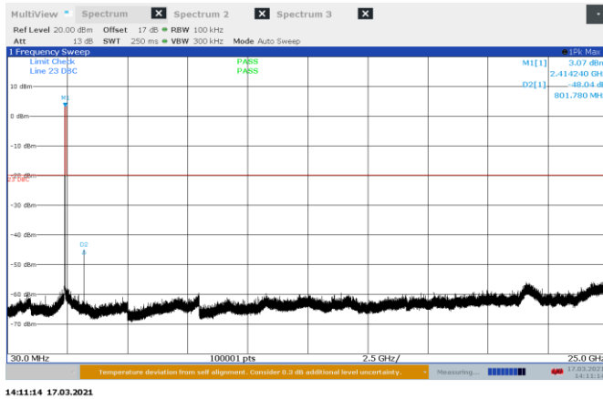
Figure 8.7-26: Conducted spurious emissions on 802.11b, Port A 2412 MHz
