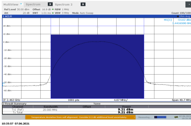
Figure 8.6-1: Conducted output power on 802.11b, sample plot
