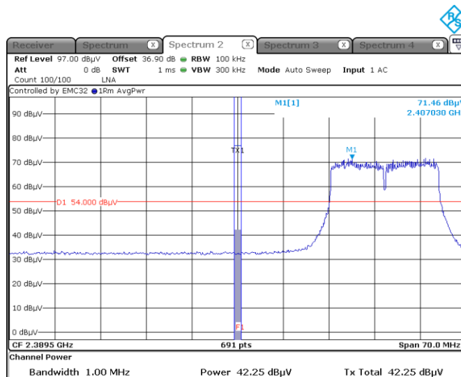
Figure 8.7-6: Radiated restricted-band band edge at 2390 MHz, 802.11g Average
