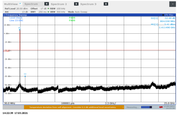
Figure 8.7-27: Conducted spurious emissions on 802.11b, Port B 2412 MHz
