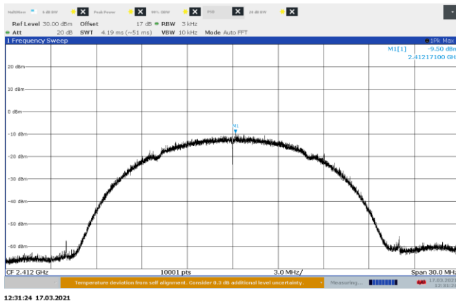
Figure 8.8-1: Conducted PSD on 802.11b, sample plot
