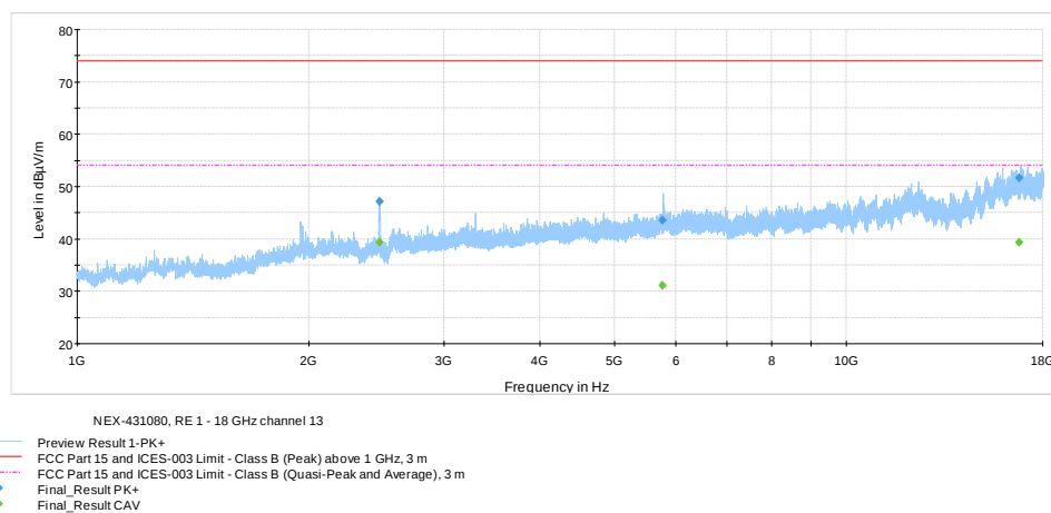
Figure 8.7-14: Radiated spurious emissions 1 – 18 GHz on 802.11b @ 2472 MHz
