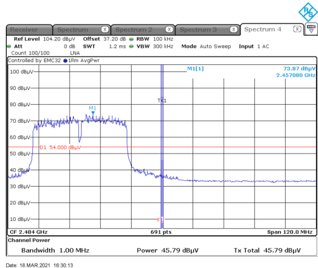
Figure 8.7-4: Radiated restricted-band band edge at 2483.5 MHz, 802.11n HT40 Average
