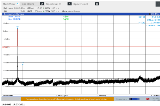
Figure 8.7-30: Conducted spurious emissions on 802.11b, Port A 2462 MHz
