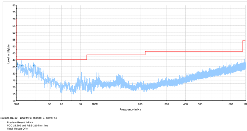
Figure 8.7-10: Radiated spurious emissions 30 – 1000 MHz on 802.11b @ 2442 MHz
