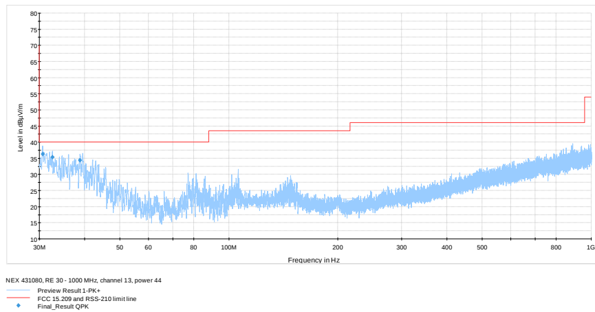
Figure 8.7-11: Radiated spurious emissions 30 – 1000 MHz on 802.11b @ 2472 MHz
