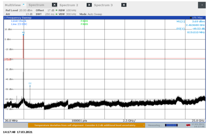
Figure 8.7-31: Conducted spurious emissions on 802.11b, Port B 2462 MHz
