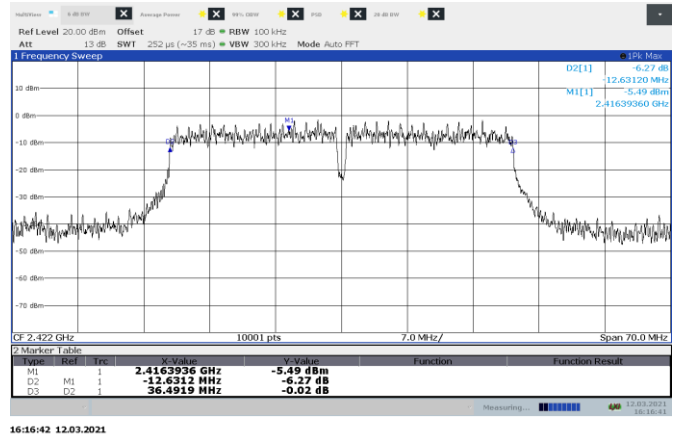
Figure 8.5-4: 6 dB bandwidth on 802.11n HT40, sample plot
