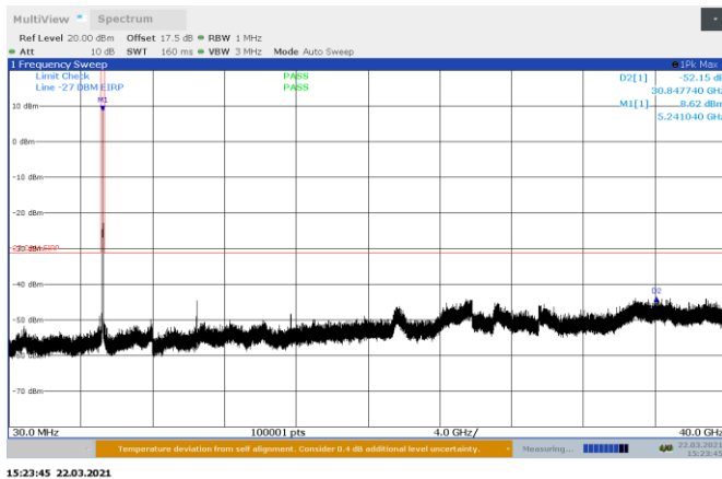
Figure 8.8-11: Conducted spurious emissions on 802.11a, high channel Port A
