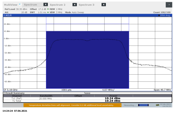
Figure 8.7-2: Conducted output power on 802.11a, Port B Low channel
