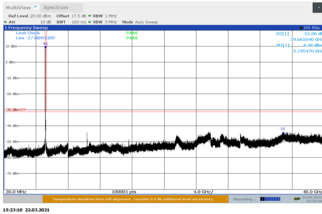
Figure 8.8-9: Conducted spurious emissions on 802.11a, mid channel Port A
