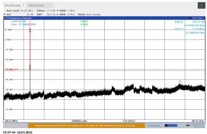
Figure 8.8-18: Conducted spurious emissions on 802.11ac, high channel Port B
