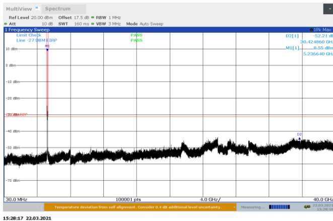
Figure 8.8-17: Conducted spurious emissions on 802.11a, high channel Port B
