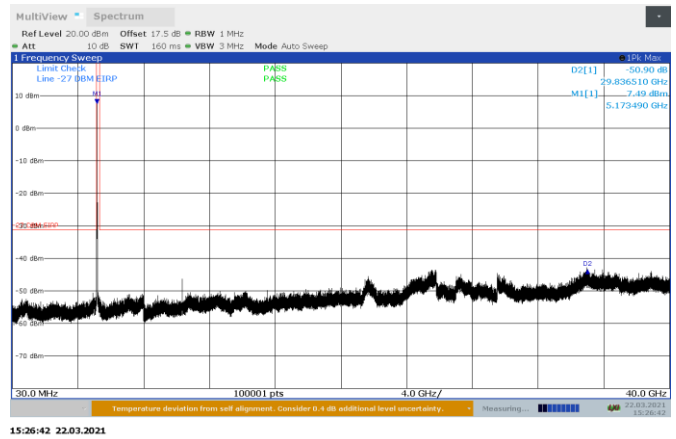
Figure 8.8-14: Conducted spurious emissions on 802.11ac, low channel Port B
