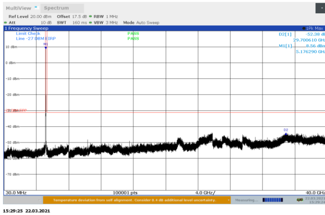
Figure 8.8-13: Conducted spurious emissions on 802.11a, low channel Port B
