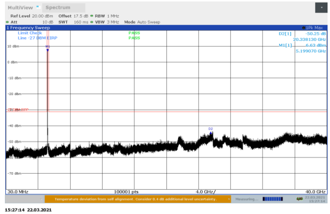
Figure 8.8-16: Conducted spurious emissions on 802.11ac, mid channel Port B
