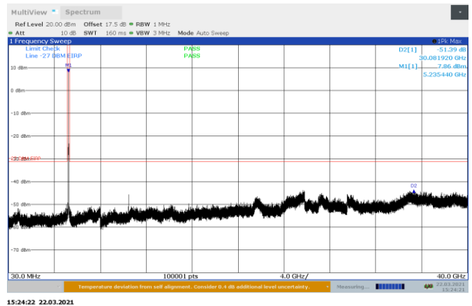
Figure 8.8-12: Conducted spurious emissions on 802.11ac, high channel Port A
