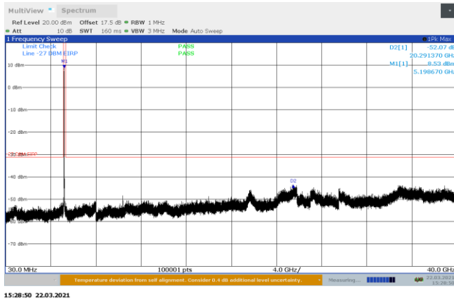
Figure 8.8-15: Conducted spurious emissions on 802.11a, mid channel Port B
