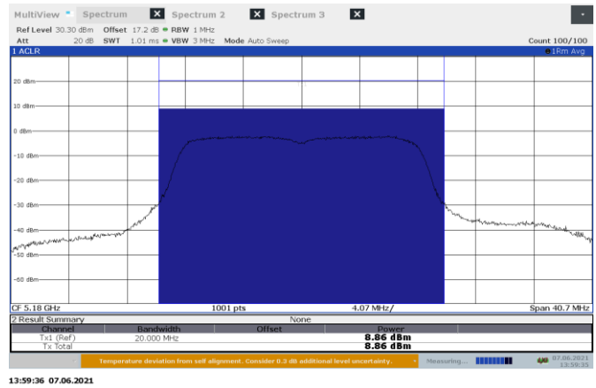
Figure 8.7-8: Conducted output power on 802.11ac, Port B Low channel
