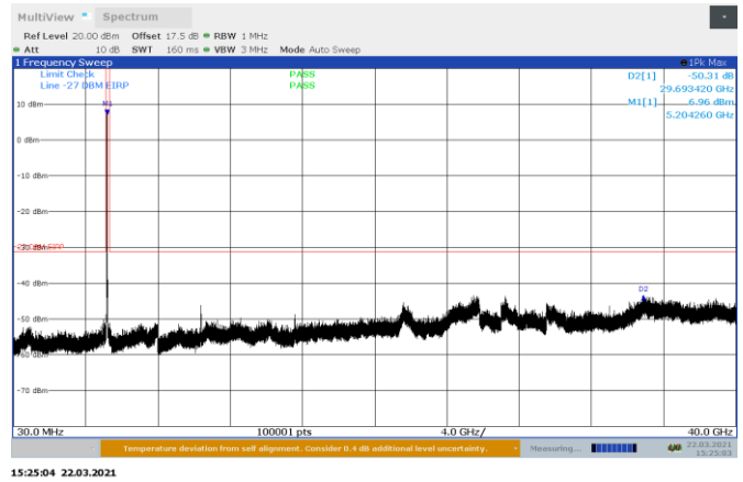
Figure 8.8-10: Conducted spurious emissions on 802.11ac, mid channel Port A
