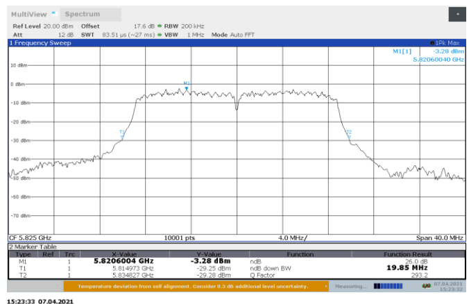
Figure 8.5-24: 26 dB bandwidth on 802.11ac, Port B High Channel
