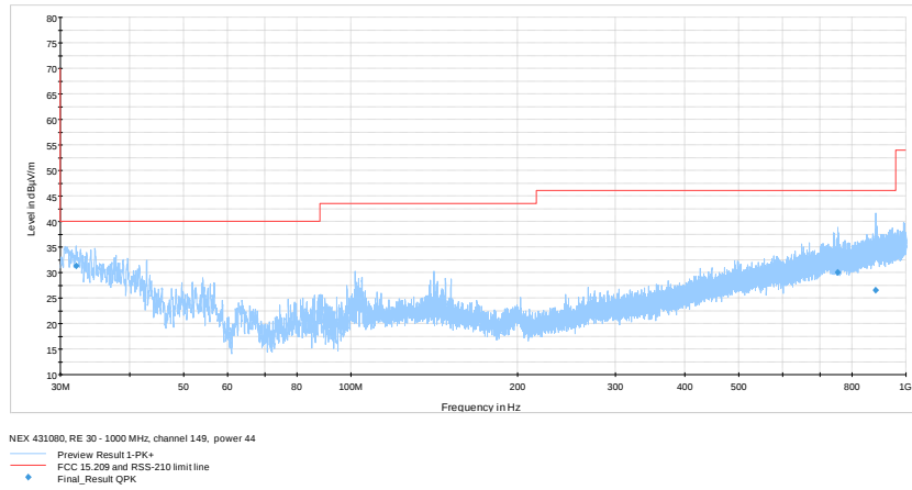
Figure 8.8-21: Radiated spurious emissions 30 – 1000 MHz on 802.11a, Low channel
