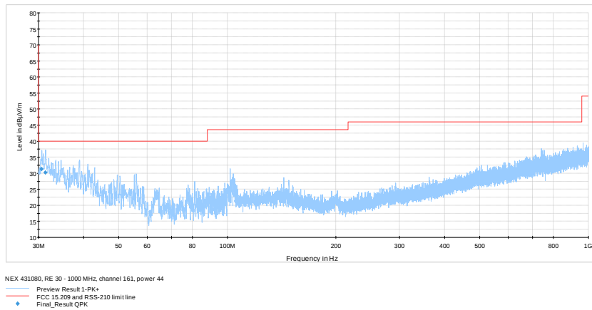
Figure 8.8-22: Radiated spurious emissions 30 – 1000 MHz on 802.11a, Mid channel
