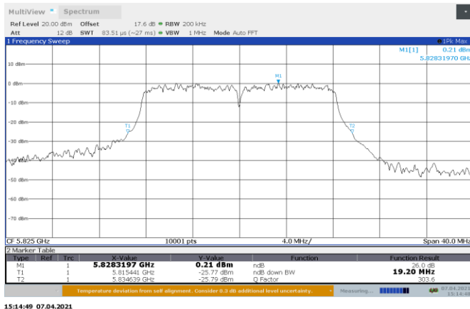
Figure 8.5-17: 26 dB bandwidth on 802.11a, Port A High Channel
