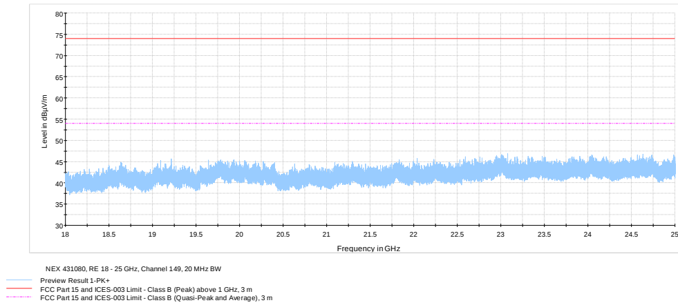
Figure 8.8-27: Radiated spurious emissions 18 – 25 GHz on 802.11a, Low channel
