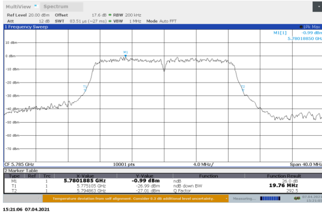
Figure 8.5-21: 26 dB bandwidth on 802.11ac, Port A Mid Channel
