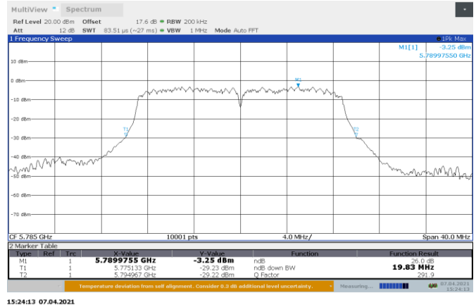
Figure 8.5-22: 26 dB bandwidth on 802.11ac, Port B Mid Channel
