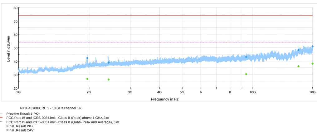
Figure 8.8-26: Radiated spurious emissions 1 – 18 GHz on 802.11a, High channel
