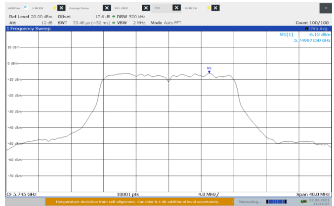
Figure 8.7-14: Conducted PSD on 802.11a, Port B Low Channel
