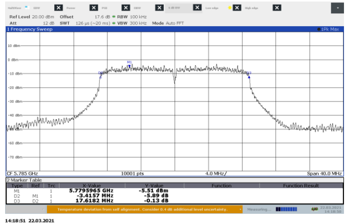
Figure 8.5-10: 6 dB bandwidth on 802.11ac, Port B Mid Channel
