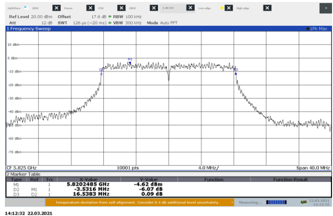
Figure 8.5-6: 6 dB bandwidth on 802.11a, Port B High Channel
