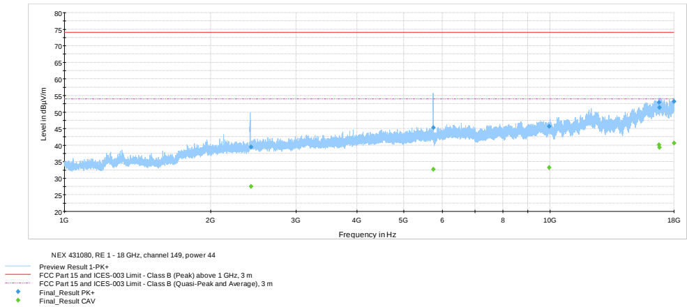
Figure 8.8-24: Radiated spurious emissions 1 – 18 GHz on 802.11a, Low channel
