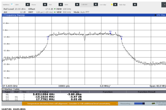
Figure 8.5-11: 6 dB bandwidth on 802.11ac, Port A High Channel
