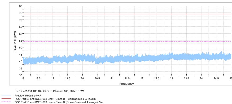
Figure 8.8-29: Radiated spurious emissions 18 – 25 GHz on 802.11a, High channel
