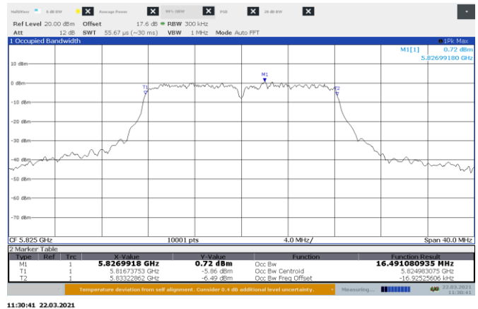
Figure 8.6-6: 99% bandwidth on 802.11a, Port B High Channel
