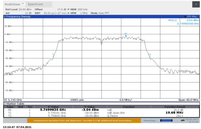
Figure 8.5-20: 26 dB bandwidth on 802.11ac, Port B Low Channel
