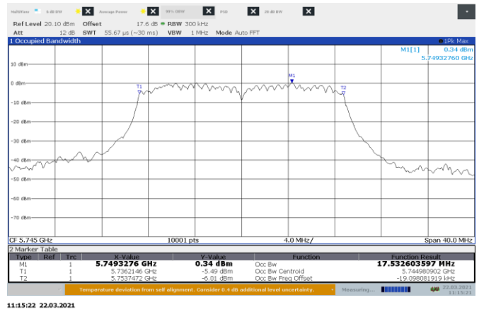
Figure 8.6-8: 99% bandwidth on 802.11ac, Port B Low Channel
