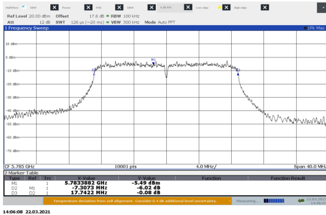
Figure 8.5-9: 6 dB bandwidth on 802.11ac, Port A Mid Channel
