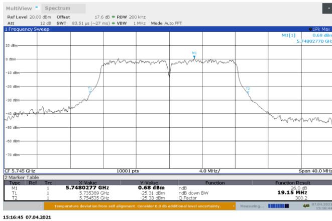
Figure 8.5-13: 26 dB bandwidth on 802.11a, Port A Low Channel
