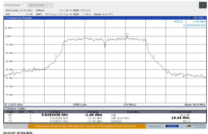
Figure 8.5-18: 26 dB bandwidth on 802.11a, Port B High Channel
