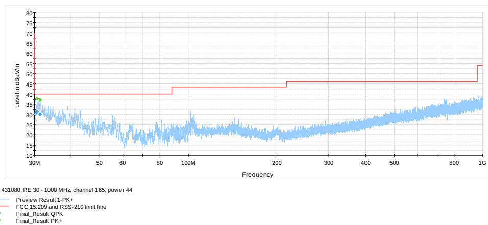
Figure 8.8-23: Radiated spurious emissions 30 – 1000 MHz on 802.11a, High channel
