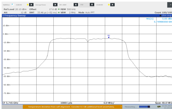
Figure 8.7-19: Conducted PSD on 802.11ac, Port A Low Channel
