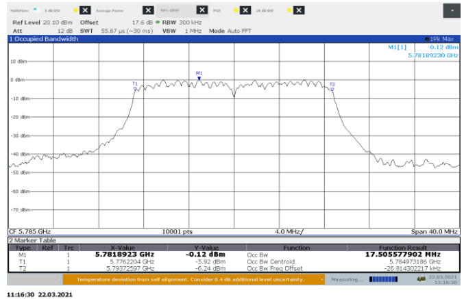
Figure 8.6-10: 99% bandwidth on 802.11ac, Port B Mid Channel
