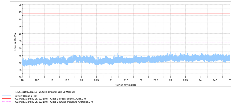
Figure 8.8-28: Radiated spurious emissions 18 – 25 GHz on 802.11a, Mid channel
