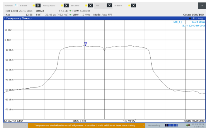
Figure 8.7-20: Conducted PSD on 802.11ac, Port B Low Channel
