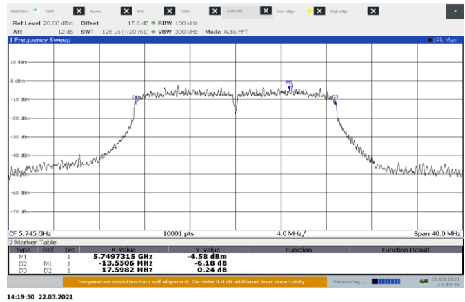
Figure 8.5-8: 6 dB bandwidth on 802.11ac, Port B Low Channel
