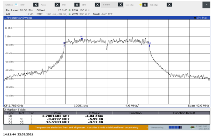
Figure 8.5-4: 6 dB bandwidth on 802.11a, Port B Mid Channel
