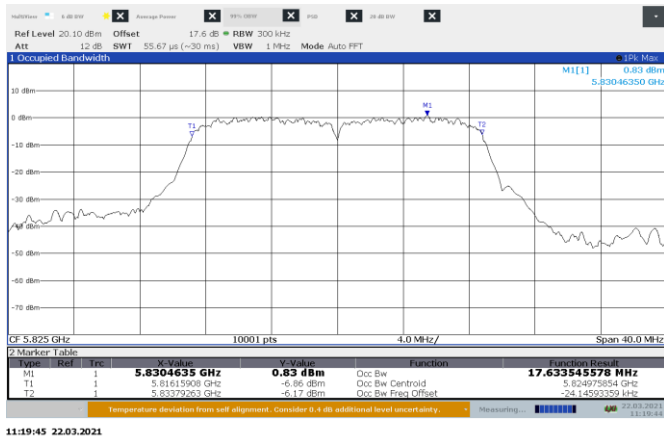
Figure 8.6-11: 99% bandwidth on 802.11ac, Port A High Channel
