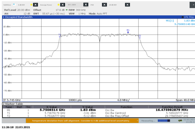
Figure 8.6-1: 99% bandwidth on 802.11a, Port A Low Channel
