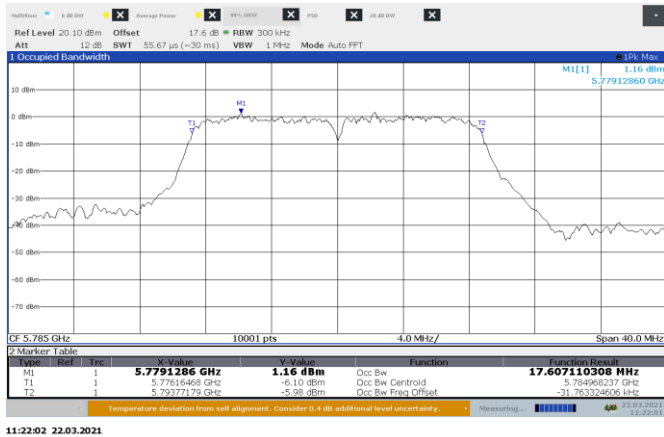
Figure 8.6-9: 99% bandwidth on 802.11ac, Port A Mid Channel
