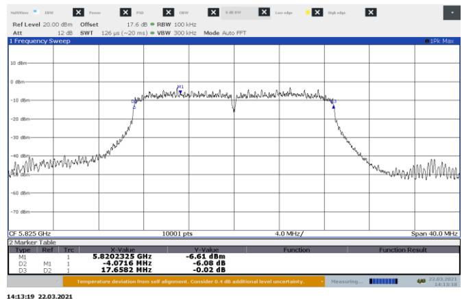
Figure 8.5-12: 6 dB bandwidth on 802.11ac, Port B High Channel
