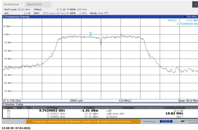
Figure 8.5-19: 26 dB bandwidth on 802.11ac, Port A Low Channel
