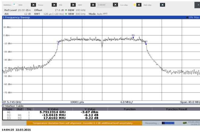
Figure 8.5-7: 6 dB bandwidth on 802.11ac, Port A Low Channel
