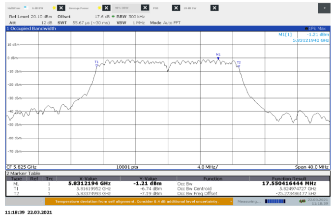
Figure 8.6-12: 99% bandwidth on 802.11ac, Port B High Channel
