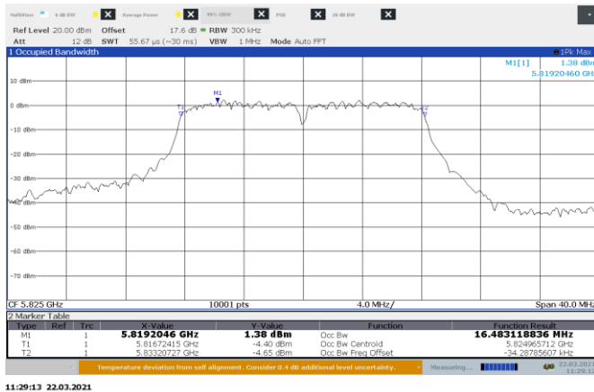
Figure 8.6-5: 99% bandwidth on 802.11a, Port A High Channel
