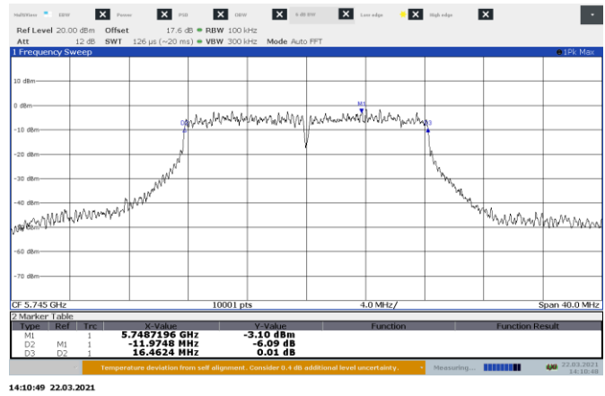
Figure 8.5-2: 6 dB bandwidth on 802.11a, Port B Low Channel
