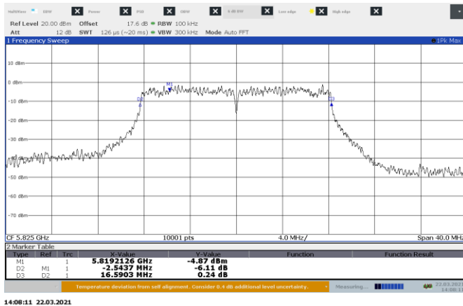
Figure 8.5-5: 6 dB bandwidth on 802.11a, Port A High Channel
