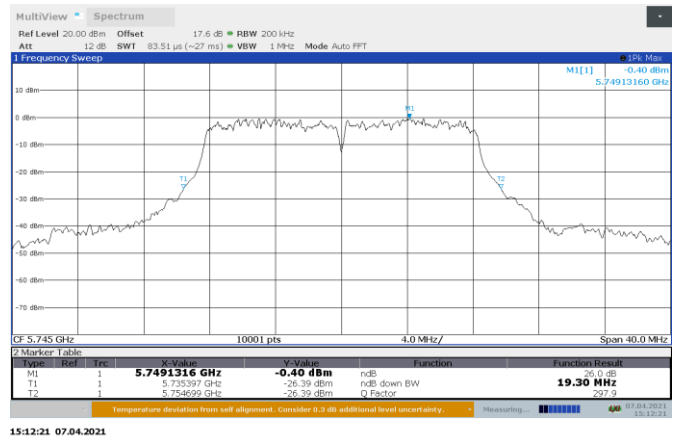
Figure 8.5-14: 26 dB bandwidth on 802.11a, Port B Low Channel
