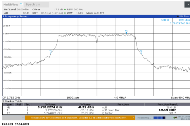
Figure 8.5-15: 26 dB bandwidth on 802.11a, Port A Mid Channel
