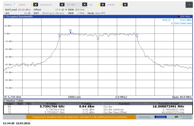
Figure 8.6-2: 99% bandwidth on 802.11a, Port B Low Channel
