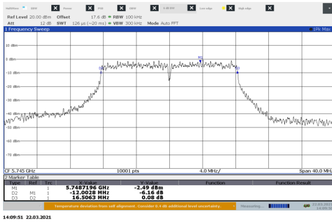
Figure 8.5-1: 6 dB bandwidth on 802.11a, Port A Low Channel
