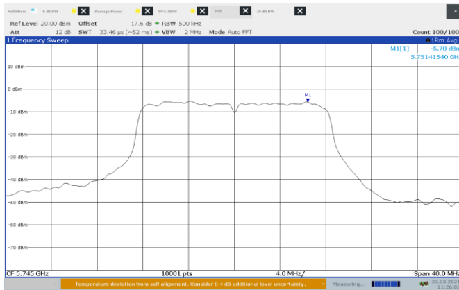
Figure 8.7-13: Conducted PSD on 802.11a, Port A Low Channel
