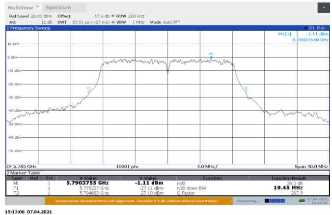
Figure 8.5-16: 26 dB bandwidth on 802.11a, Port B Mid Channel
