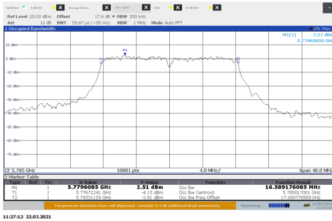
Figure 8.6-3: 99% bandwidth on 802.11a, Port A Mid Channel
