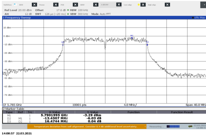
Figure 8.5-3: 6 dB bandwidth on 802.11a, Port A Mid Channel
