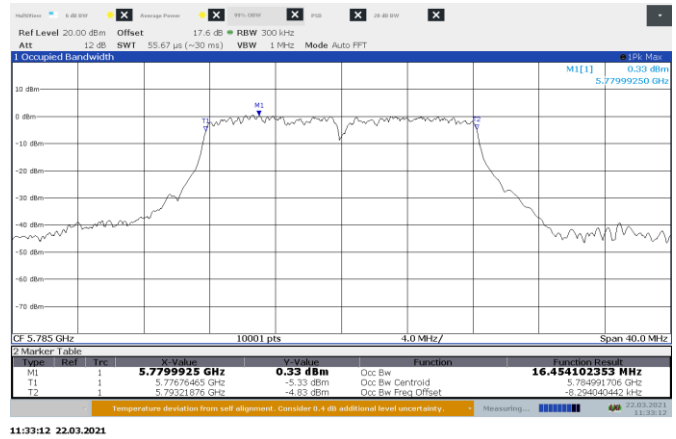
Figure 8.6-4: 99% bandwidth on 802.11a, Port B Mid Channel
