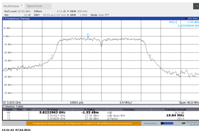
Figure 8.5-23: 26 dB bandwidth on 802.11ac, Port A High Channel
