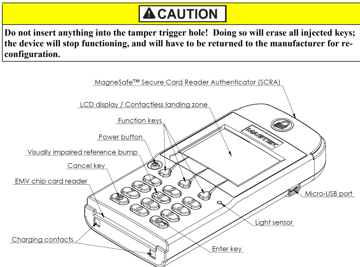
Figure 2-1 – DynaPro Go Major Components
