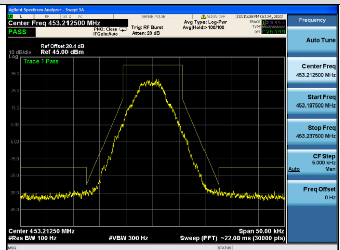
Emission Mask D@479.975MHz-10W-4FSK
