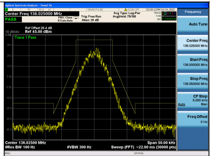
Emission Mask D@173.975MHz-10W-4FSK
