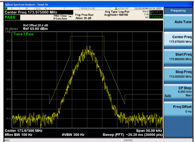
Emission Mask D@453.2125MHz-10W-4FSK
