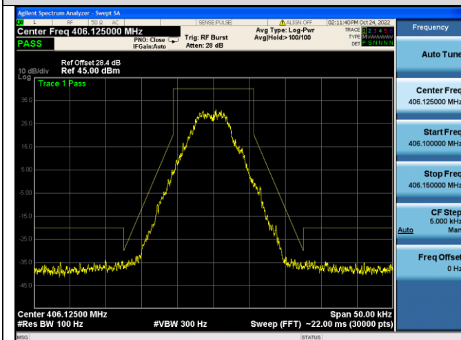
Emission Mask D@458.2125MHz-10W-4FSK
