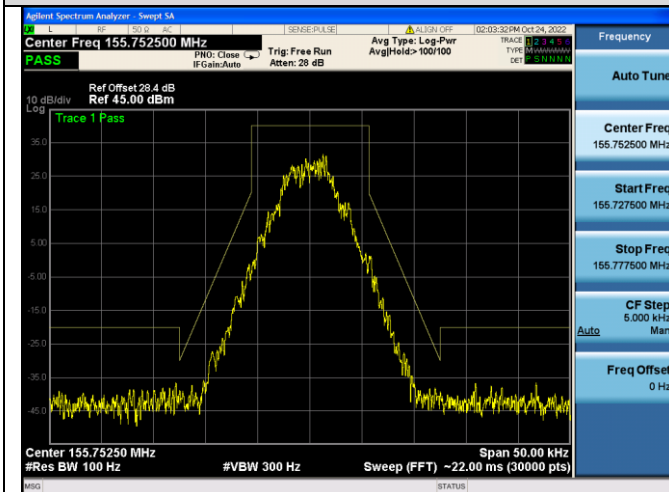
Emission Mask D@406.125MHz-10W-4FSK
