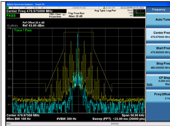
Emission Mask D@155.7525MHz-10W-4FSK
