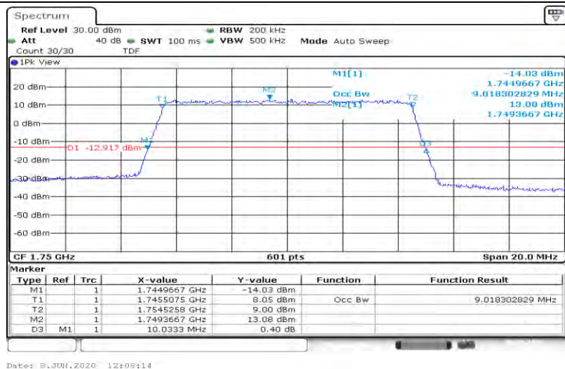
Band4-10MHz-16QAM-20000-50RB#0-9.018
