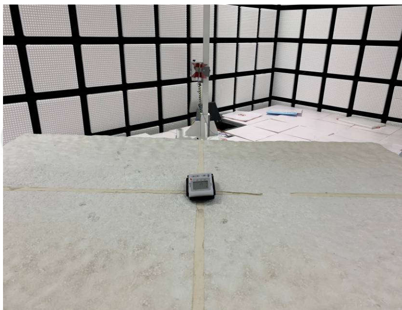
Radiated spurious emission Test Setup-3(Above 1GHz)
