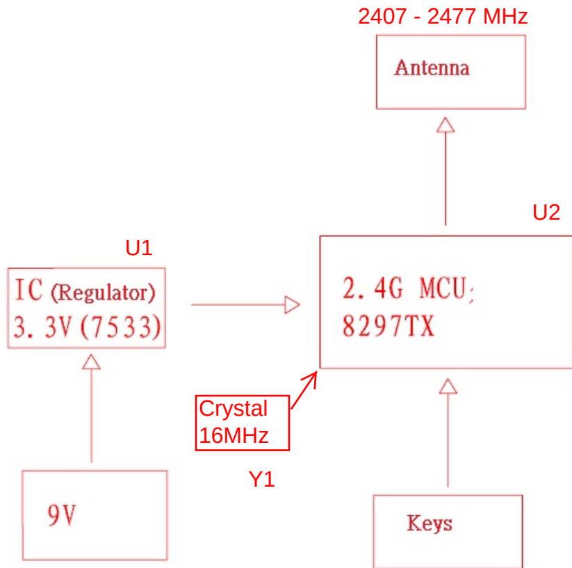
Block Diagram of HS2282- TX
