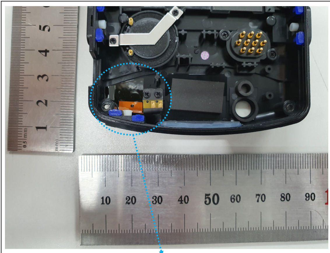
<2.4G WLAN/BT Antenna>
