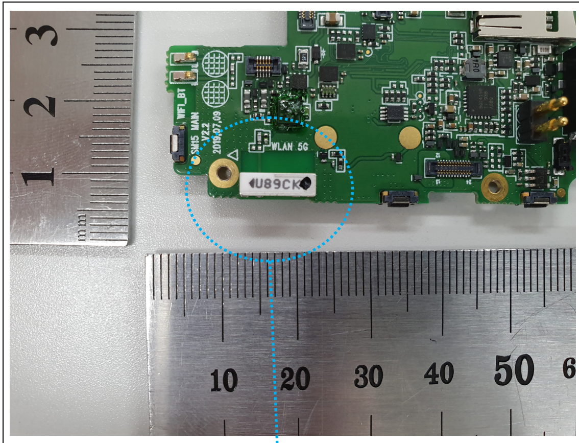
<5G WLAN Antenna>
