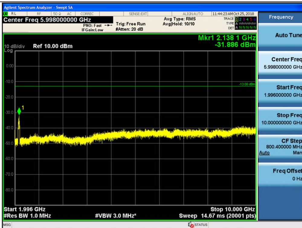
Spurious / Broadband PCS / Downlink / CDMA / Middle / High edge ~ 10 GHz
