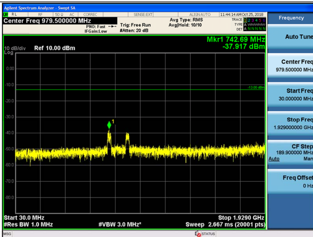
Spurious / Broadband PCS / Downlink / CDMA / Middle / 30 MHz ~ Low edge
