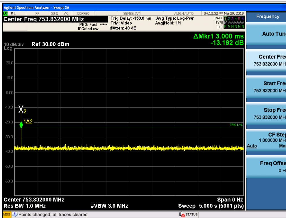
Oscillation Detect / Upper 700 MHz / Downlink
