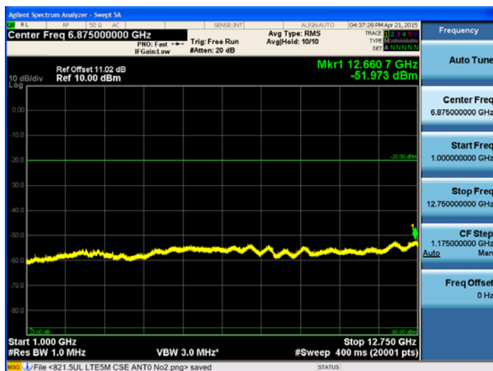
800 MHz band (1 GHz – 12.75 GHz) LTE 5MHz
