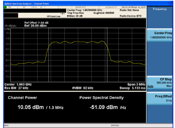
1900 MHz band CDMA Downlink Mid
