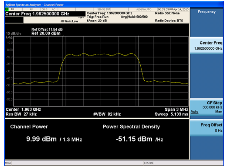
1900 MHz band CDMA EVDO Downlink Mid
