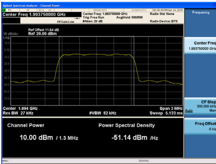
1900 MHz band CDMA Downlink High
