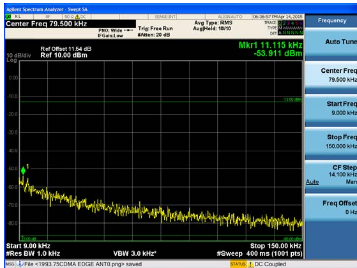
1900 MHz band (9 kHz – 150 kHz) CDMA High
