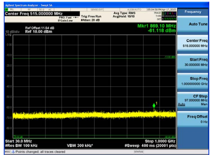
1900 MHz band (30 MHz- 1 GHz) LTE 5MHz Mid
