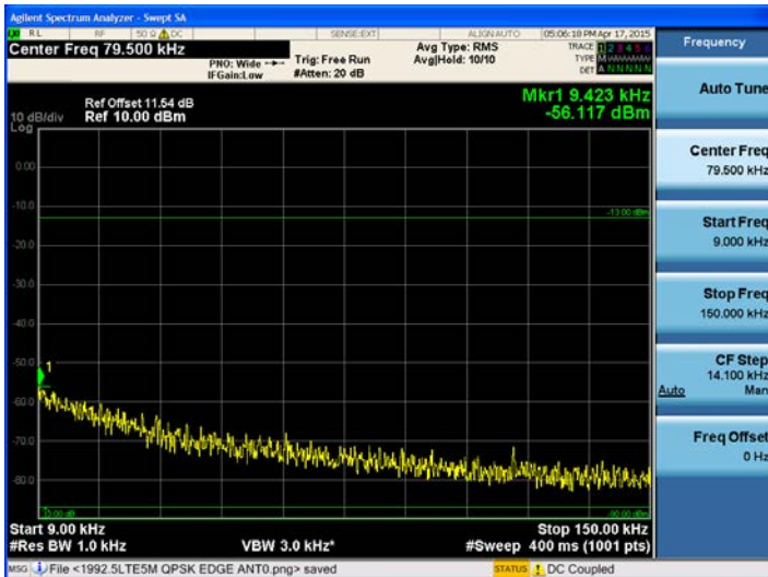
1900 MHz band (9 kHz – 150 kHz) LTE 5MHz High
