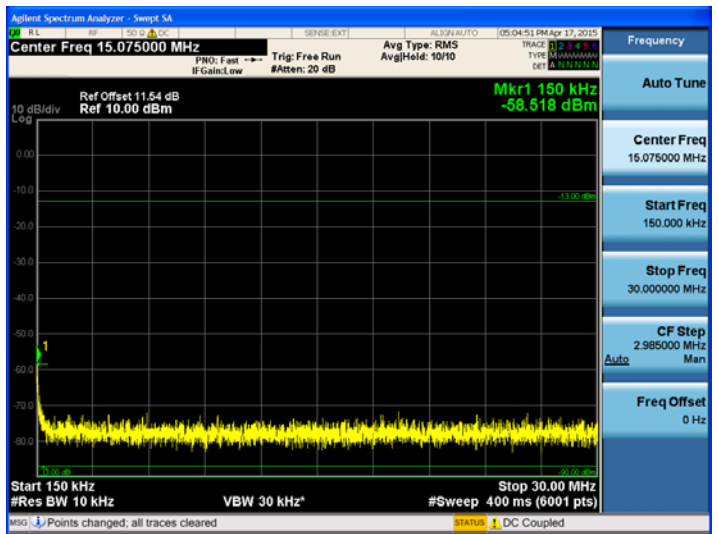
1900 MHz band (150 kHz – 30 MHz) LTE 5MHz Mid
