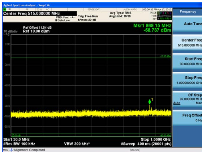
1900 MHz band (30 MHz- 1 GHz) LTE 5MHz High
