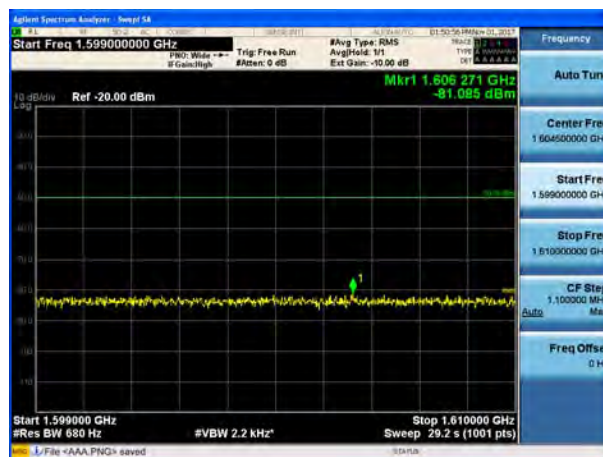
1599 MHz ~ 1610 MHz (2)
