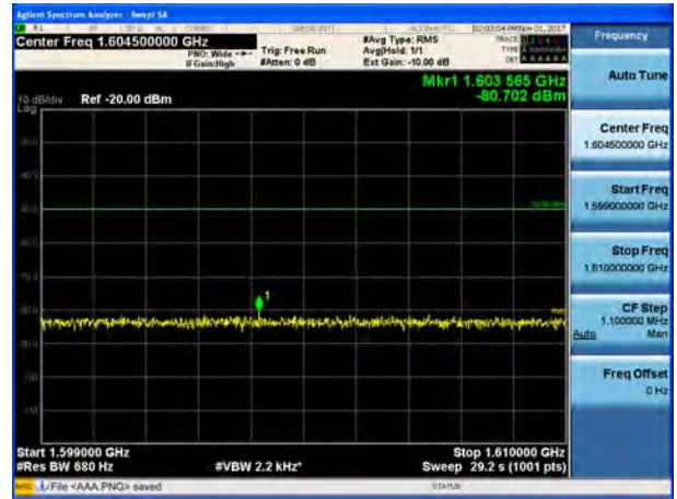
1599 MHz ~ 1610 MHz (2)
