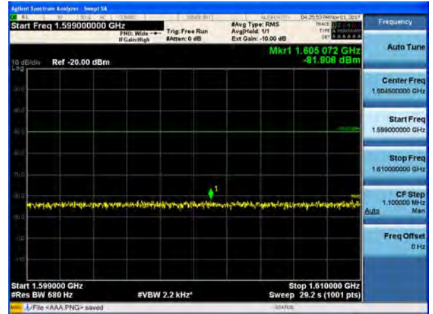
1599 MHz ~ 1610 MHz (2)
