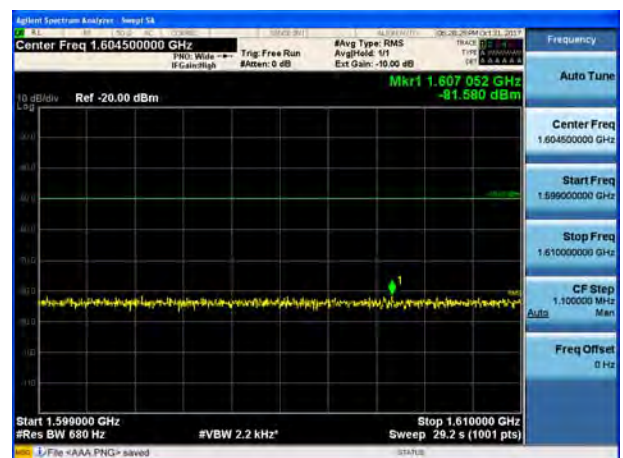
1599 MHz ~ 1610 MHz (2)
