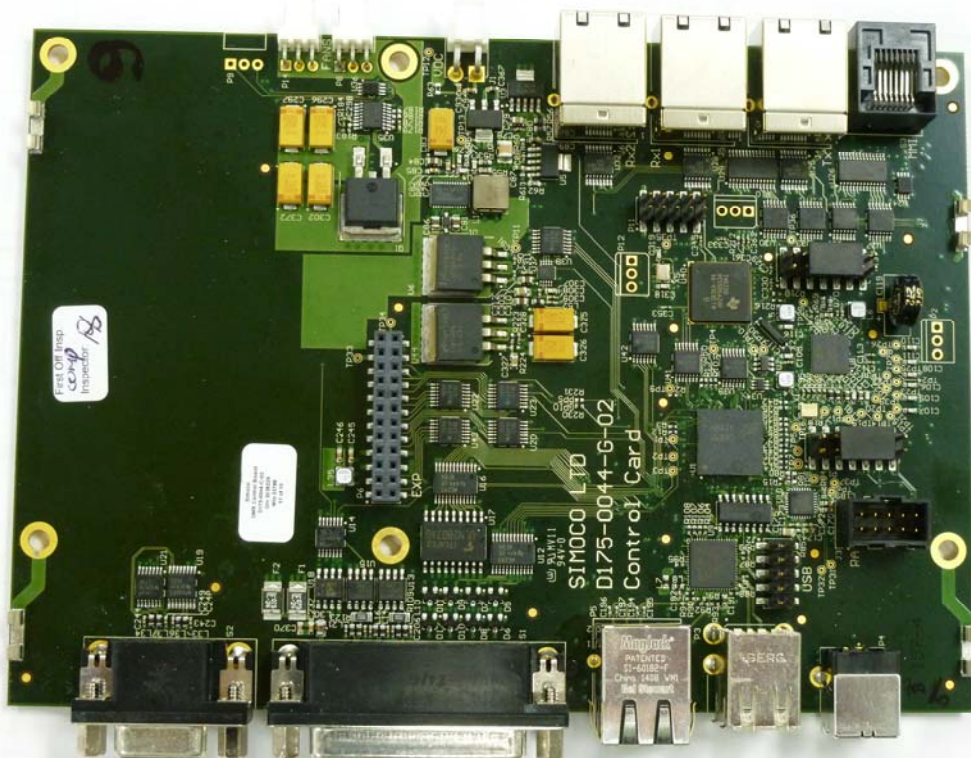
Control board top
