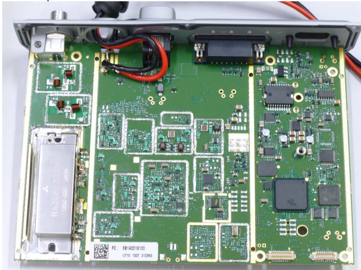
Receiver top no shields
