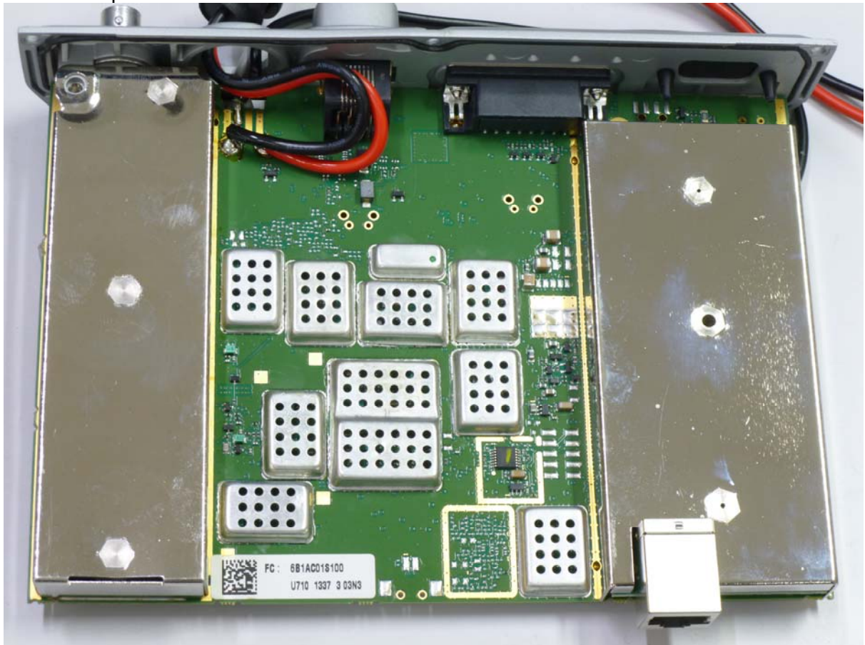
Receiver top with shields
