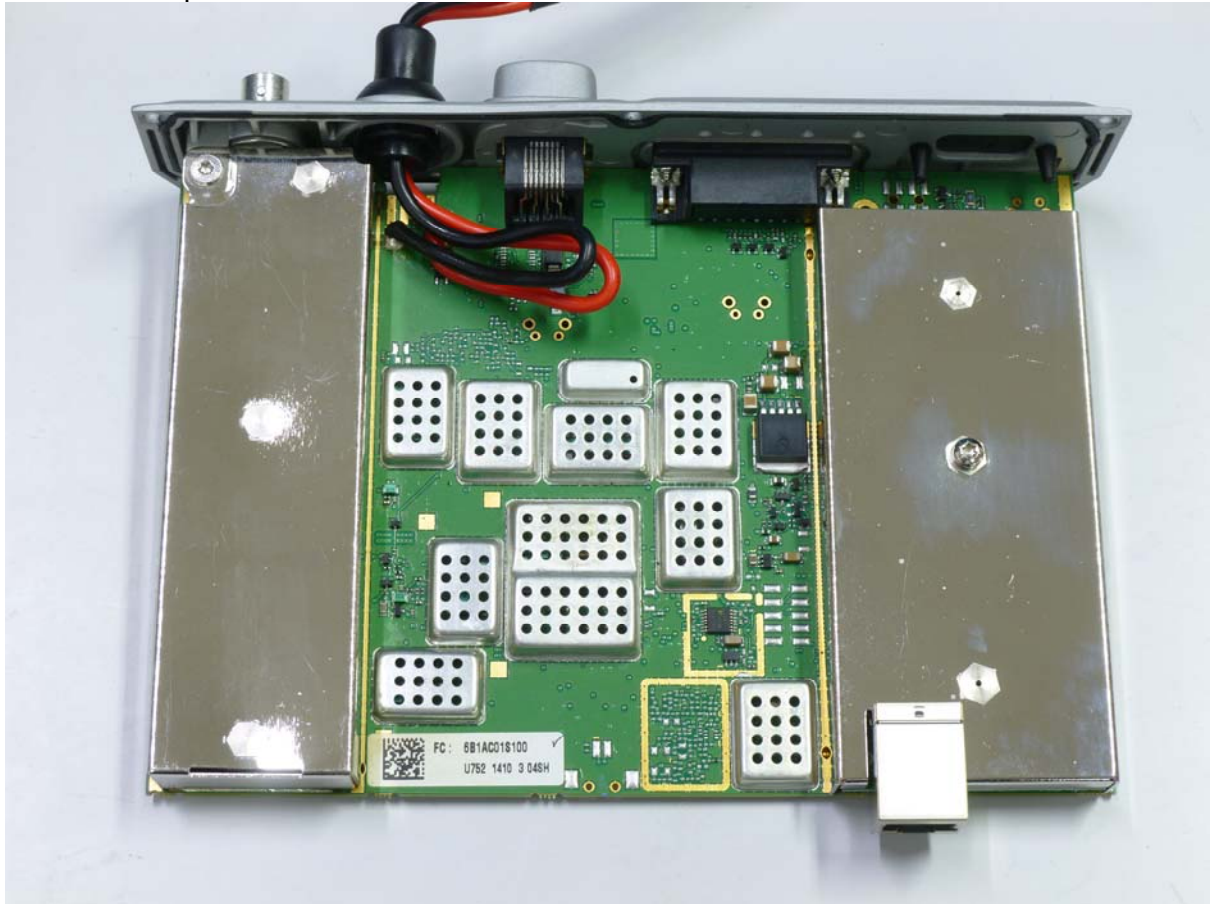
Transmitter top no covers
