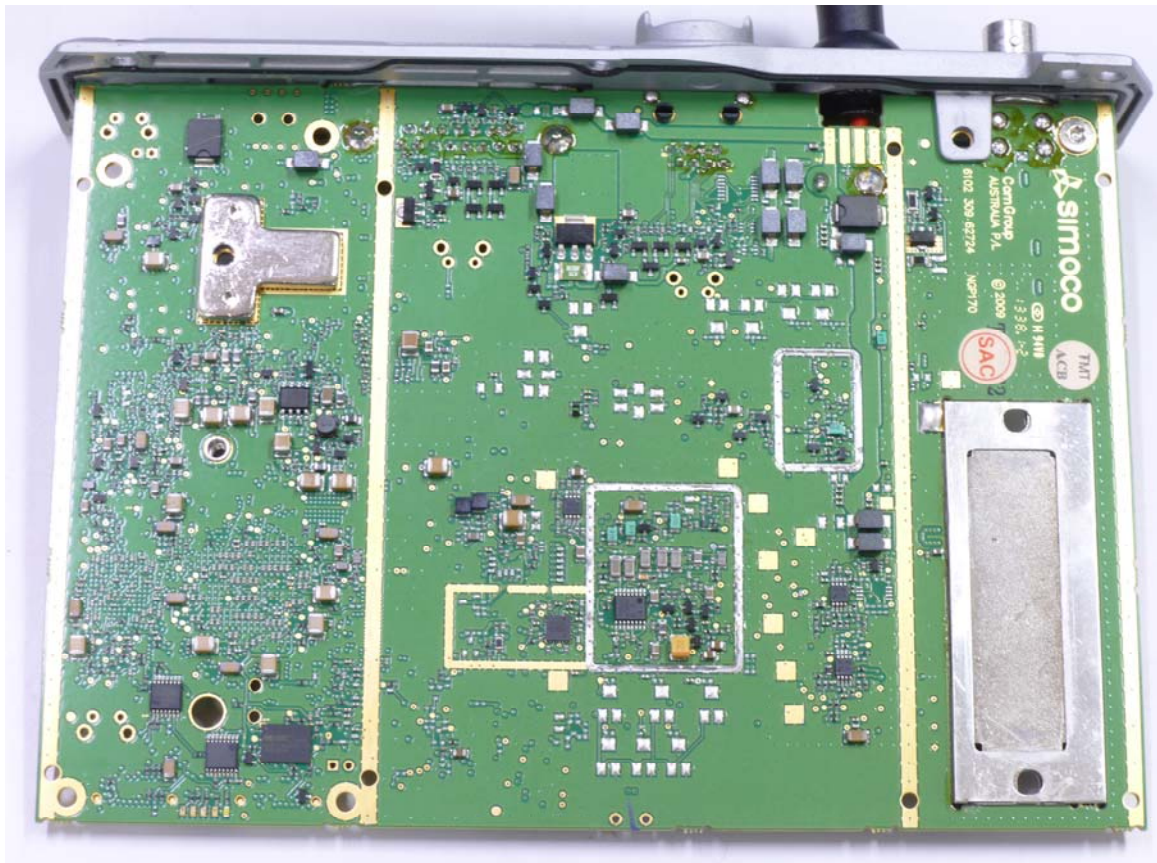
Transmitter bottom no shields
