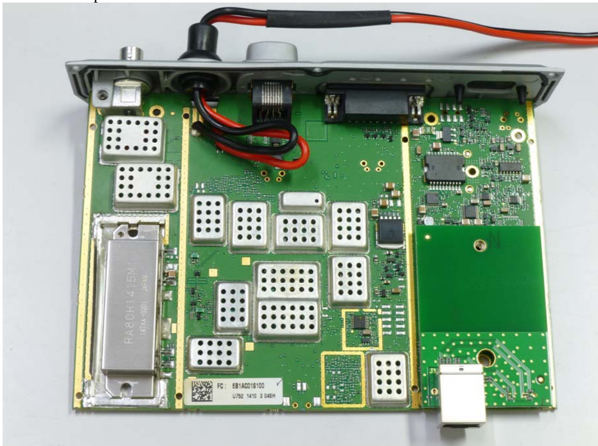
Transmitter top no covers
