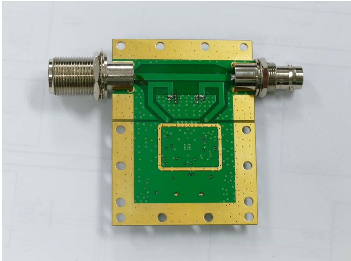
VSWR detector top no shield
