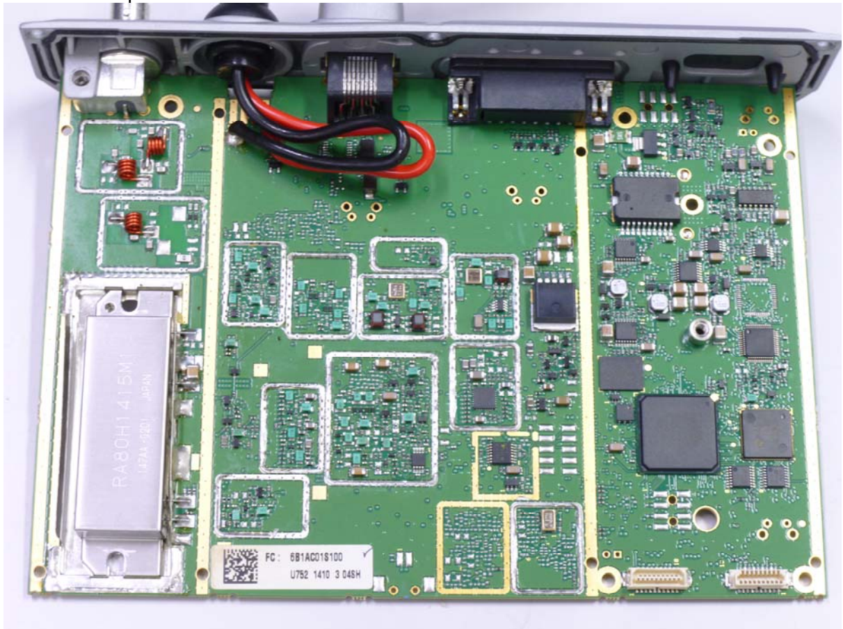
Transmitter top no shields
