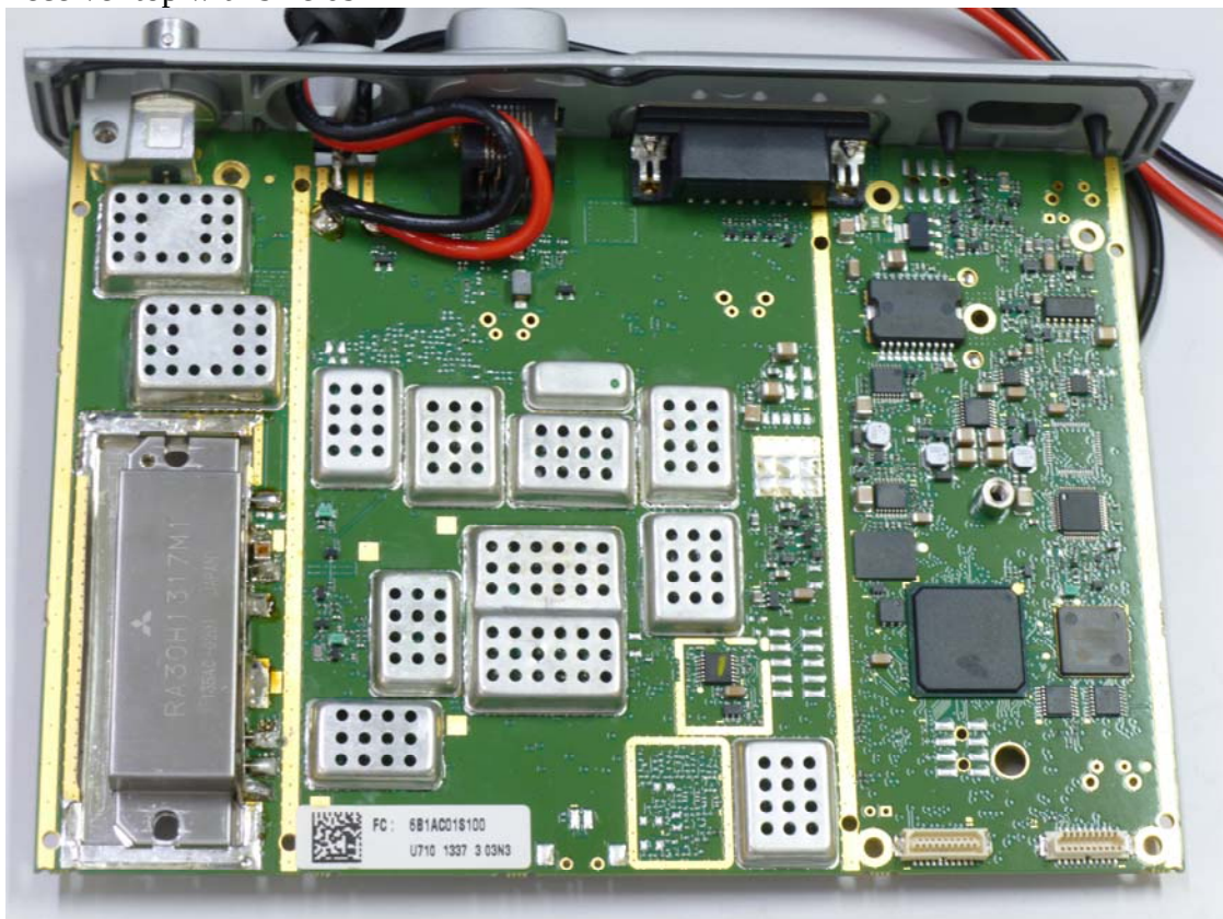
Receiver top with shields
