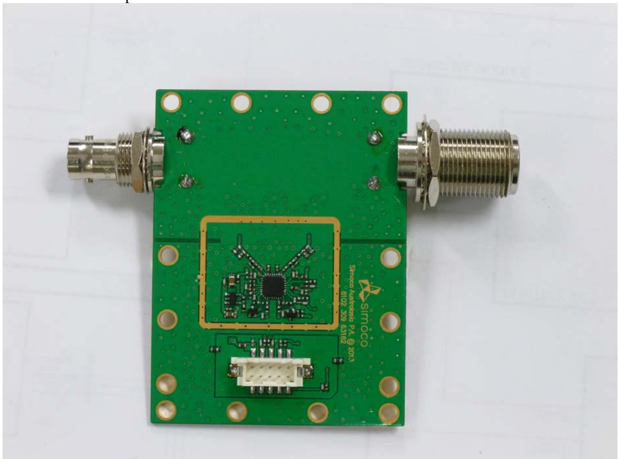
VSWR detector top no shield
