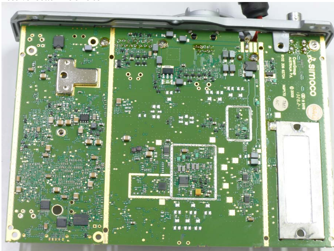
Receiver bottom no shields
