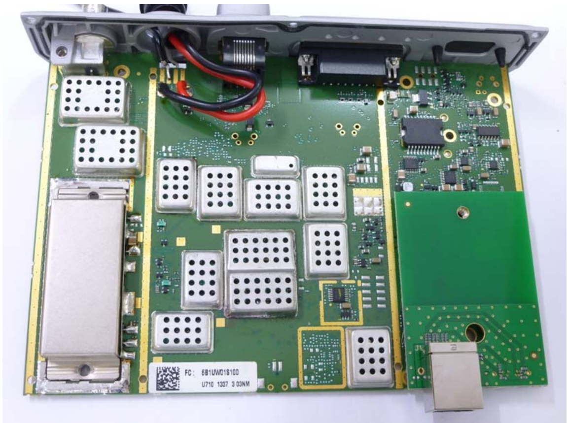
SDB680UW RX pcb Top No Covers
