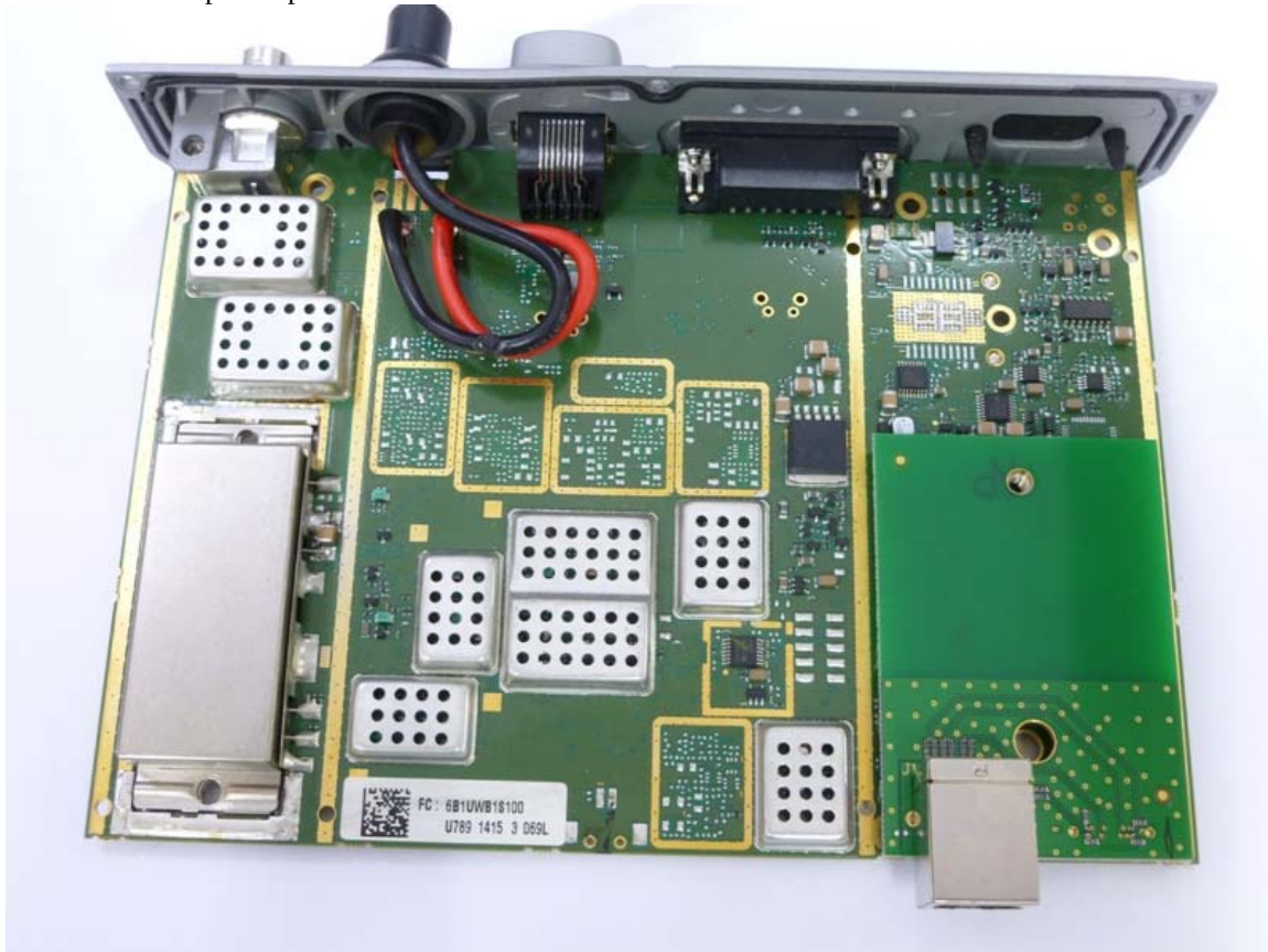
SDB680UW TX pcb Top No Covers
