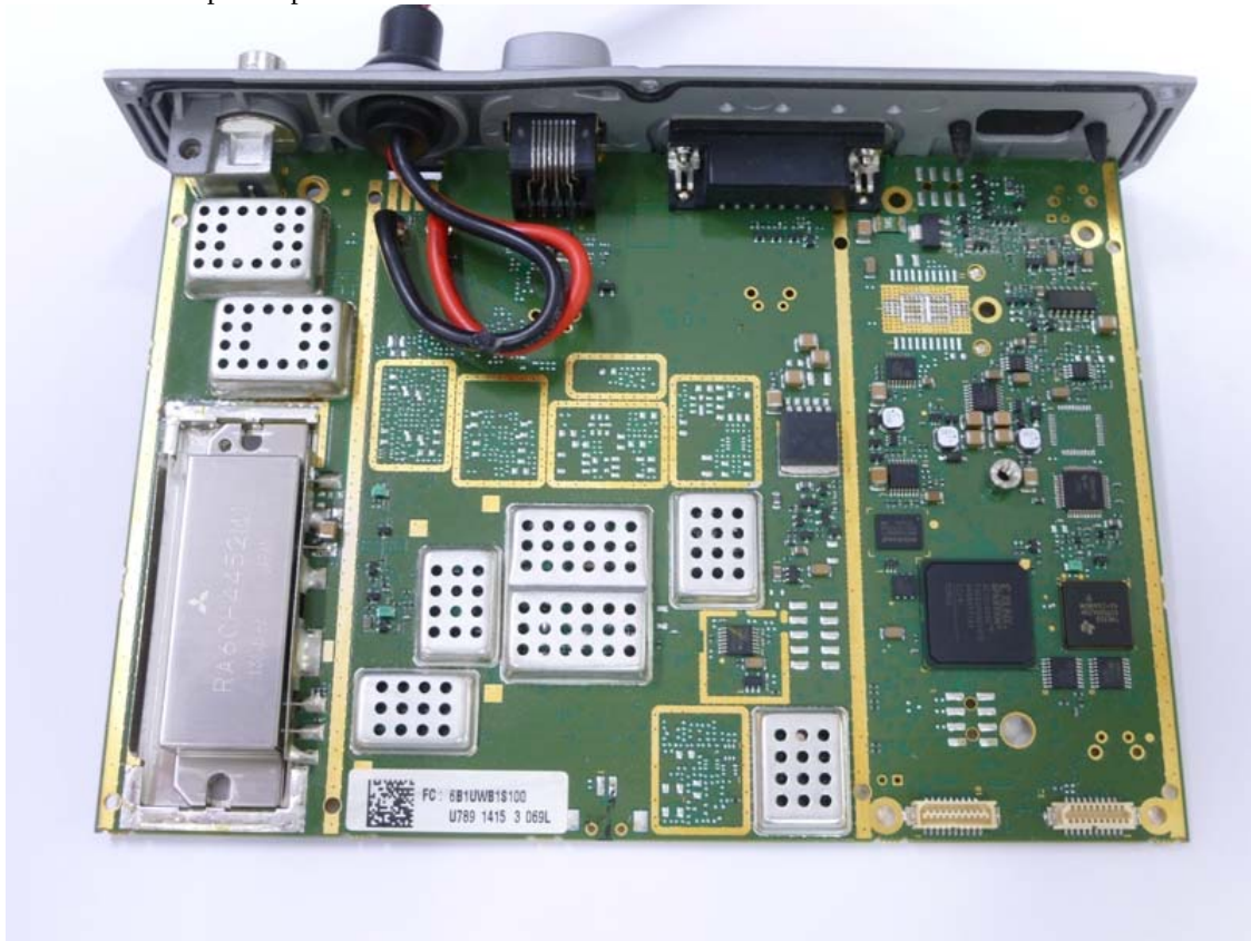
SDB680UW TX pcb Top No Interface Board
