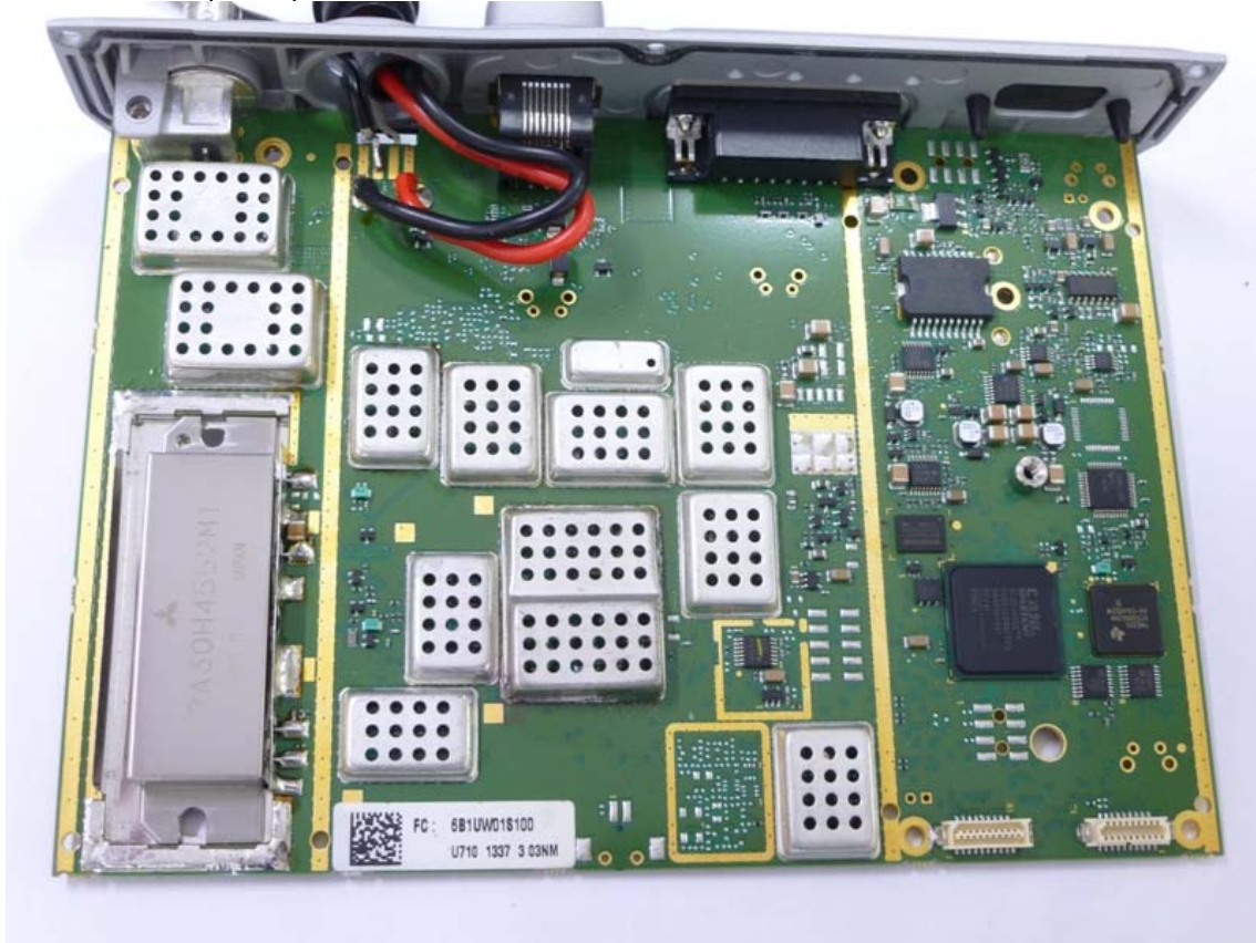
SDB680UW RX pcb Top No Interface Board
