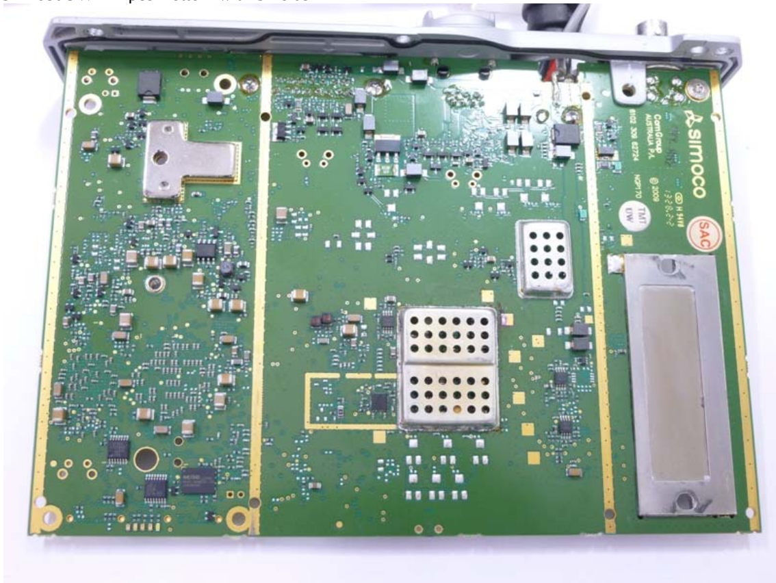
SDB680UW RX pcb Bottom with Shields
