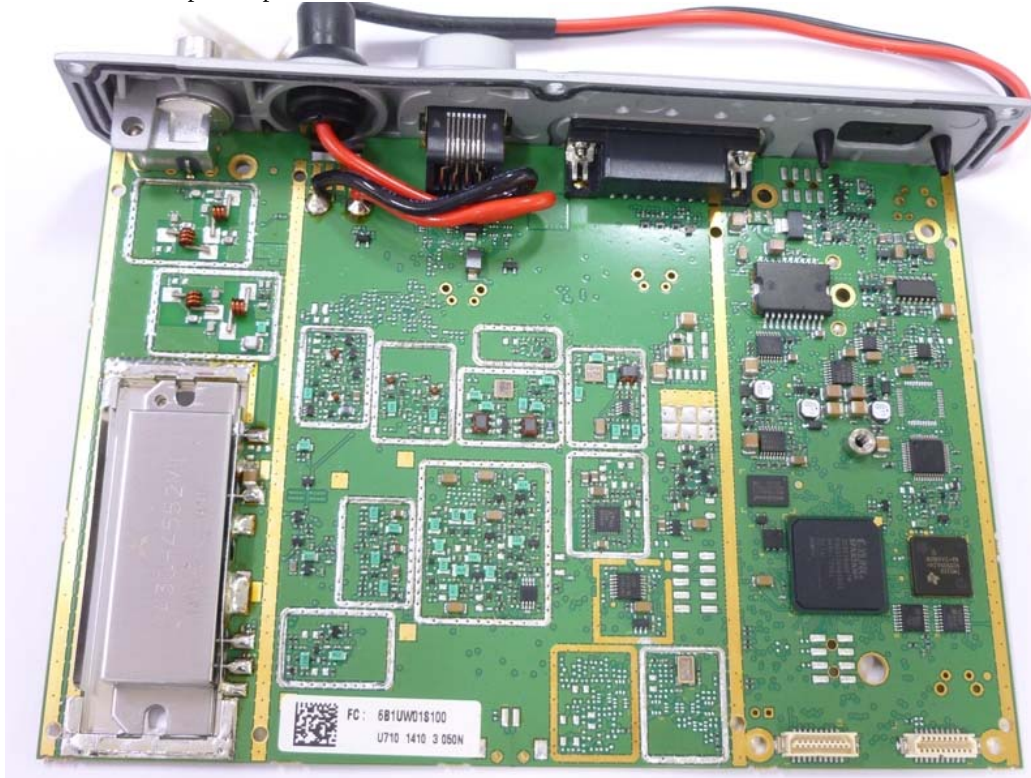
SDB680UW RX pcb Top No Shields
