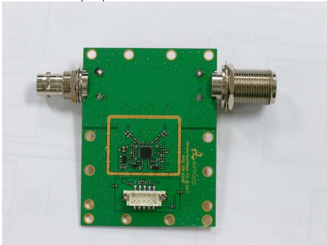
SDB680 VSWR Detector pcb Top no Shield
