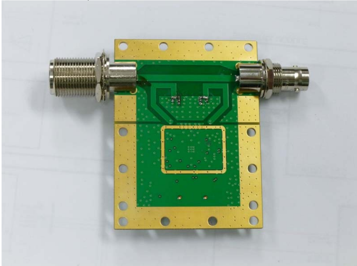
SDB680 VSWR Detector pcb Top with Shield
